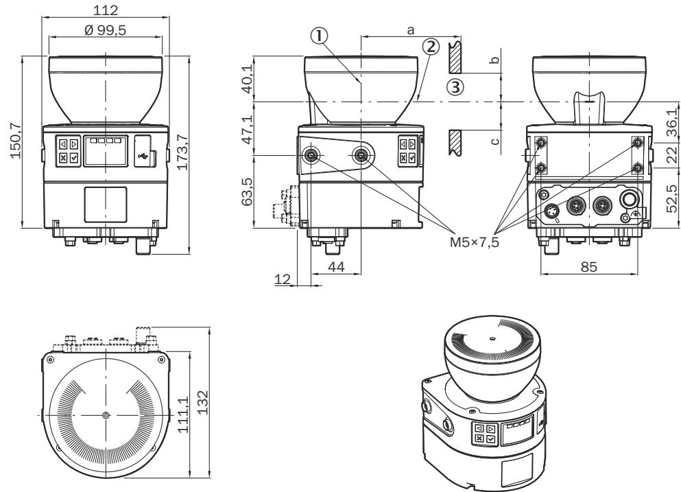
Figure 92: Dimensional drawing
