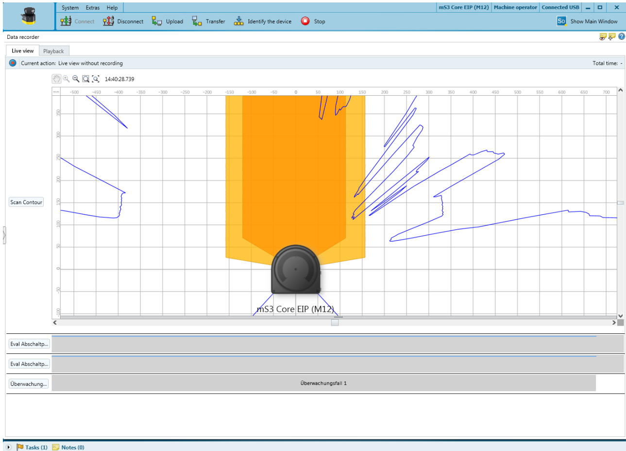
Figure 85: Data recorder
