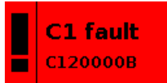
Figure 84: Error display
