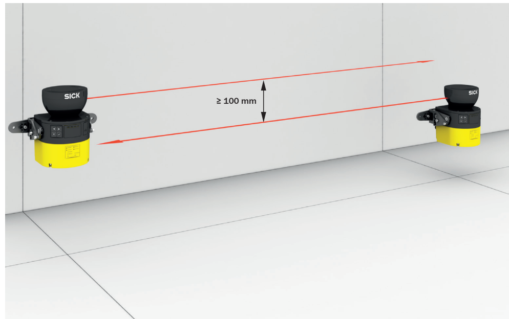
Figure 93: Mounting 2 safety laser scanners with the optics cover facing upward
