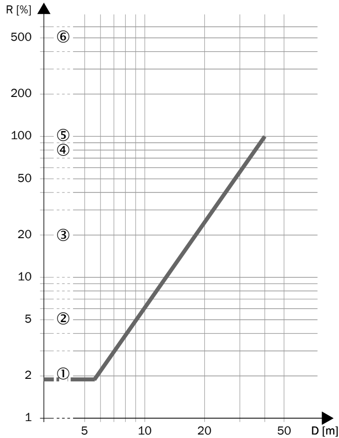
Figure 90: Scanning range and required remission for warning fields (devices with a max. protective field range of 4.0 m and devices with max. protective field range of 5.5 m)
