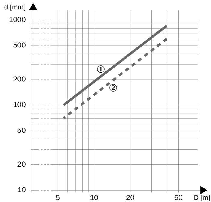
Figure 88: Scanning range and object size for warning fields (devices with a max. protective field range of 4.0 m and devices with max. protective field range of 5.5 m)
