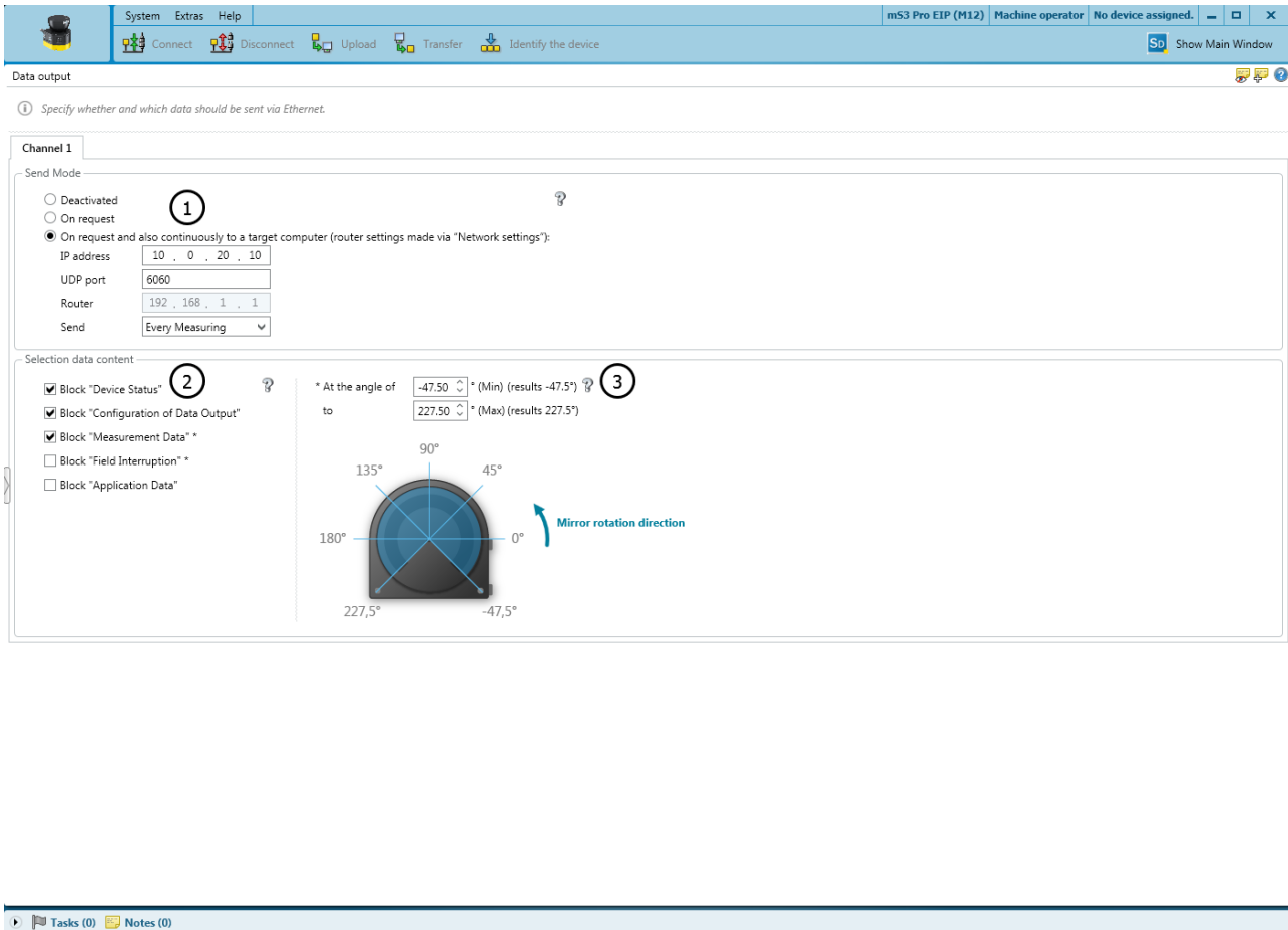
Figure 73: Data output
