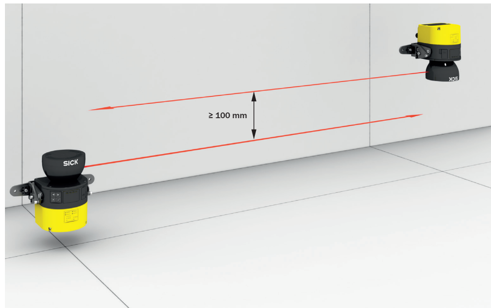
Figure 96: Mounting the upper safety laser scanner with the optics cover facing downward and mounting the lower safety laser scanner with the optics cover facing upward
