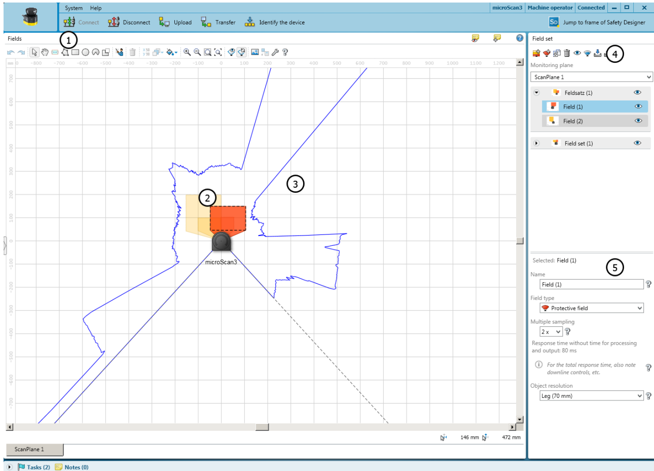
Figure 64: Field editor
