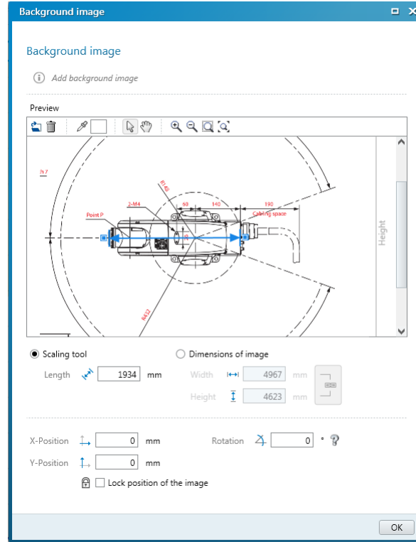
Figure 66: Background image
