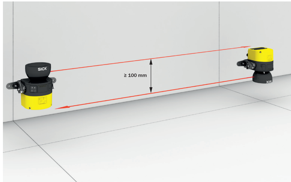
Figure 95: Mounting the upper safety laser scanner with the optics cover facing upward and mounting the lower safety laser scanner with the optics cover facing downward
