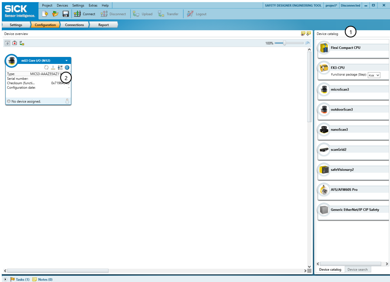
Figure 56: Configuration
