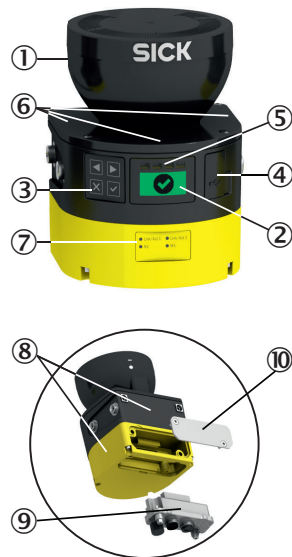
Figure 3: Device overview
