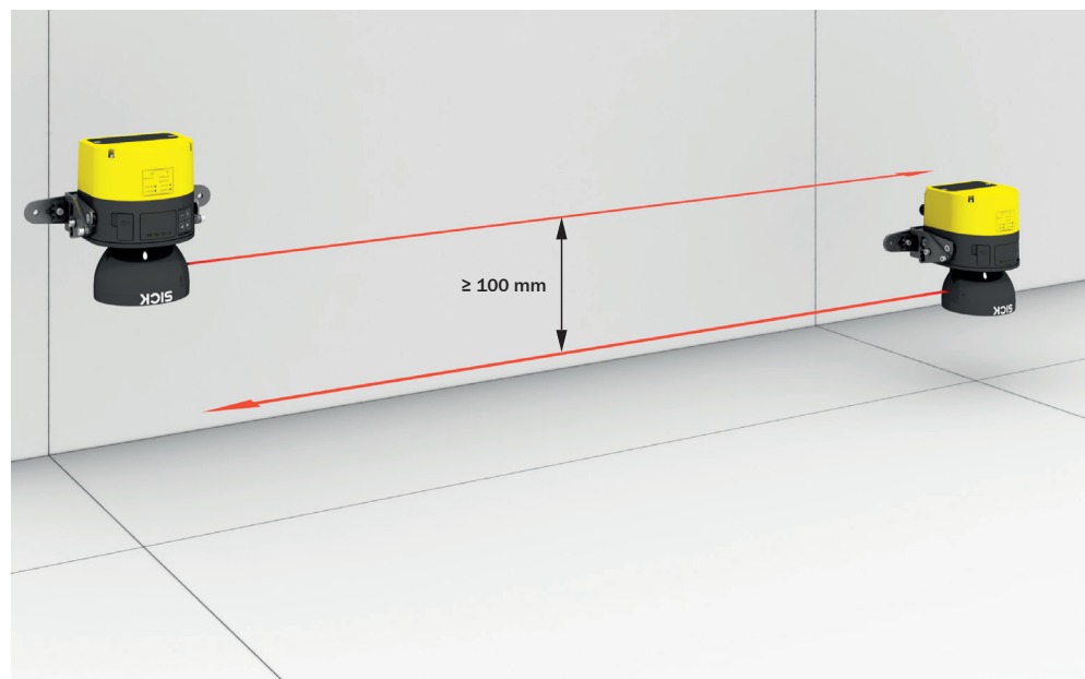
Figure 94: Mounting 2 safety laser scanners with the optics cover facing downward
