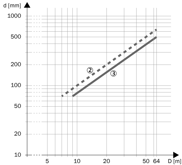
Figure 89: Scanning range and object size for warning fields (devices with a max. protective field range of 9.0 m)
