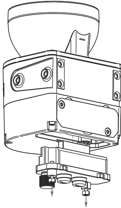
Figure 82: Replacing the system plug
