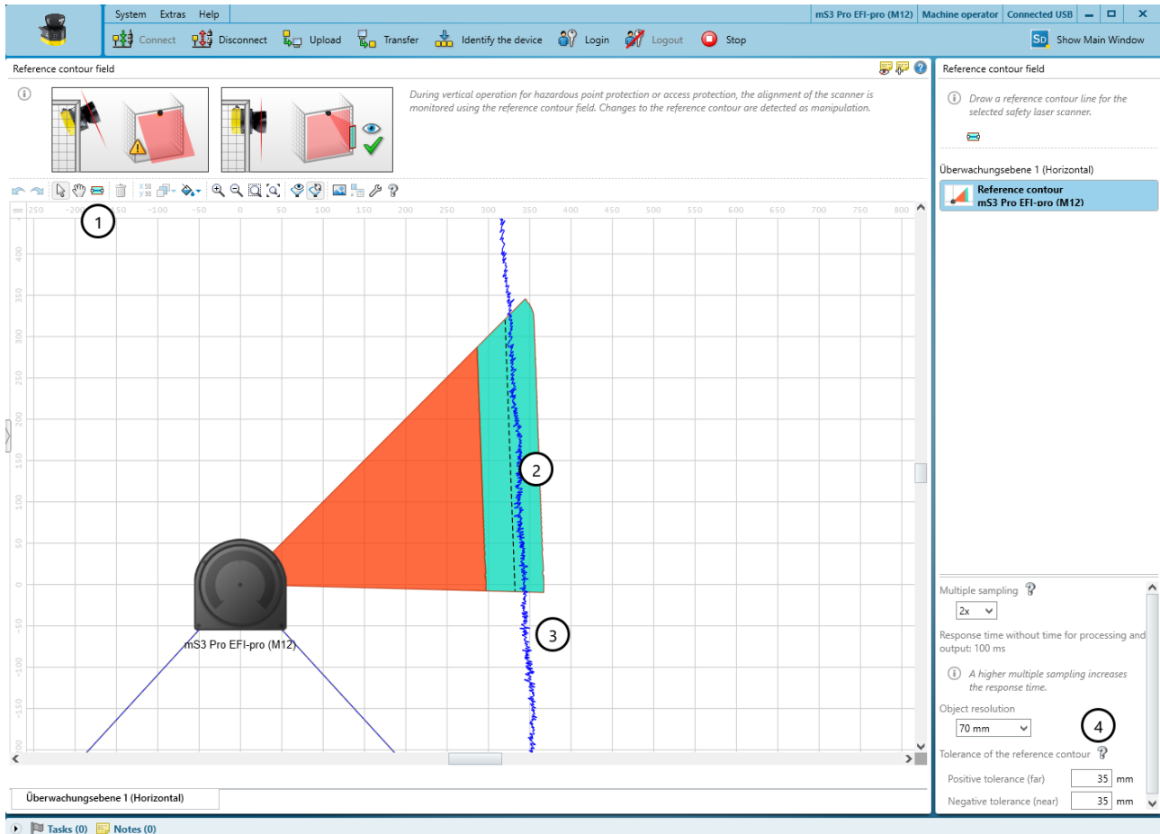
Figure 63: Reference contour field
