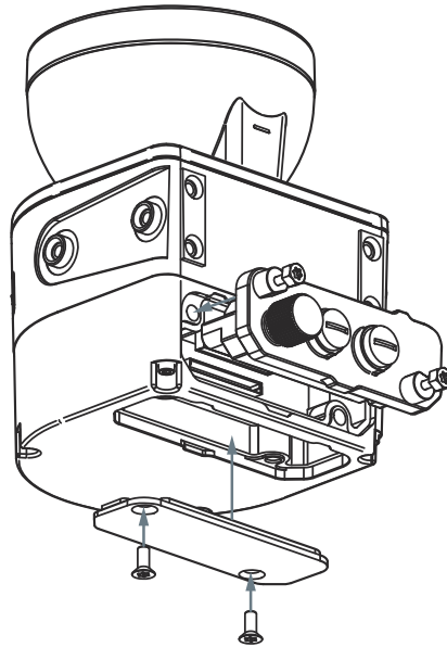
Figure 50: Installing the rear system plug
