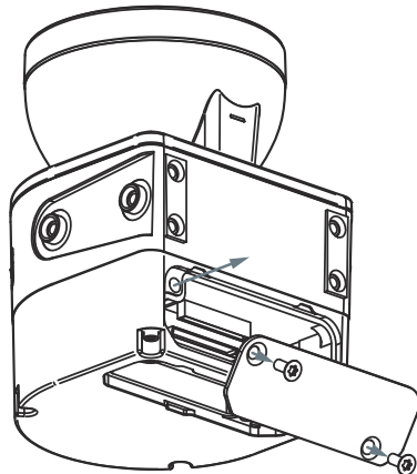
Figure 49: Remove the cover plate from the rear.
