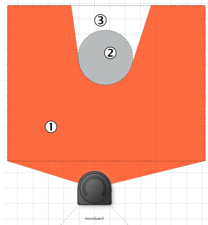
Figure 68: Area that cannot be monitored
