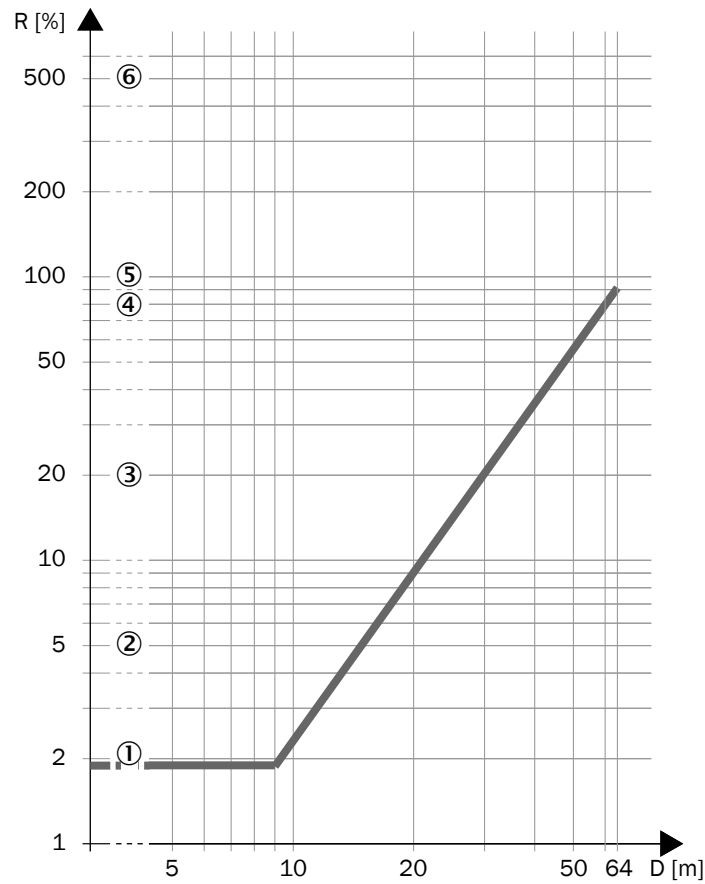
Figure 91: Scanning range and required remission for warning fields (devices with a max. protective field range of 9.0 m)
