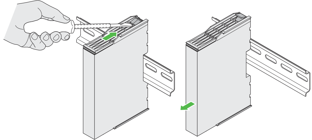
Figure 9: Disassembly
