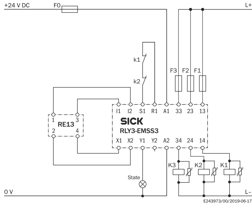
Figure 5: ReLy EMSS3 connection diagram, without restart interlock, with external device monitoring (EDM)
