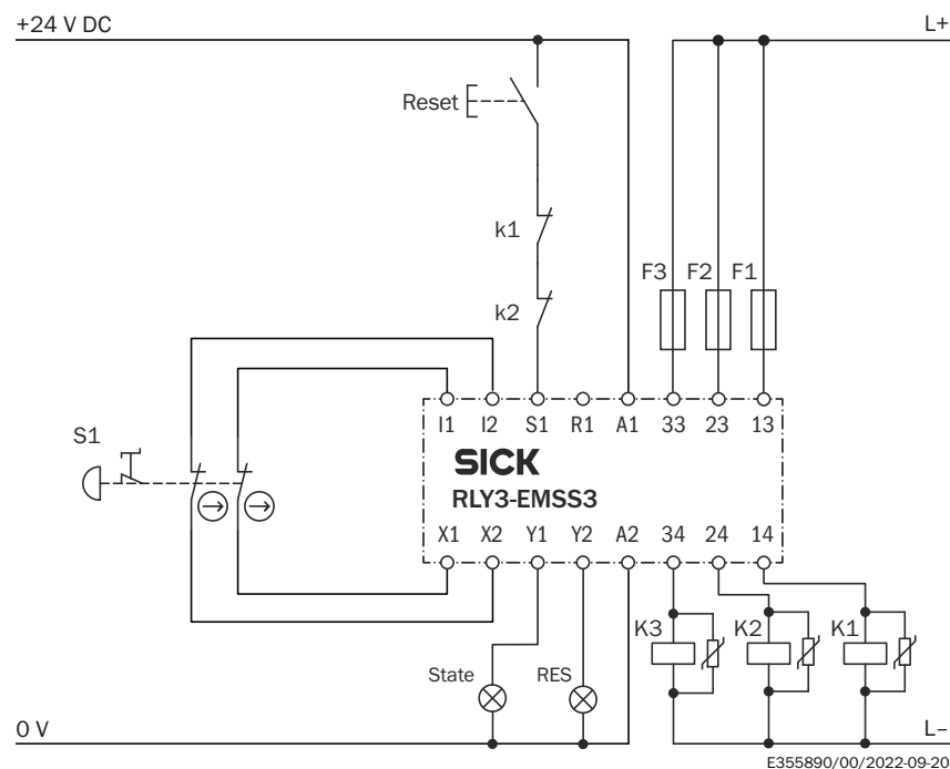
Figure 6: ReLy EMSS3 connection diagram, with restart interlock and external device monitoring (EDM)
