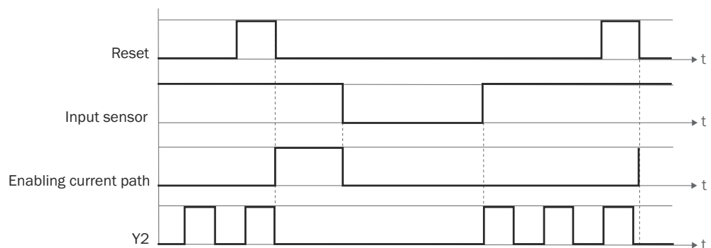
Figure 4: Sequence/timing diagram
