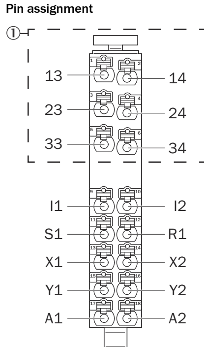
Figure 12: Terminals on front connector
