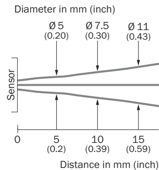
Illustration 4: GTE2F, version 15 mm
