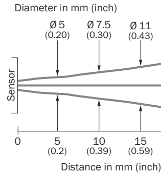
Figure 7: GTE2F, 15 mm version
