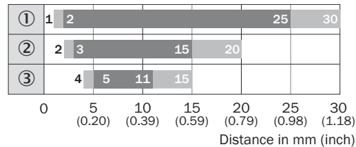
Illustration 2: Distance de commutation 15 mm
