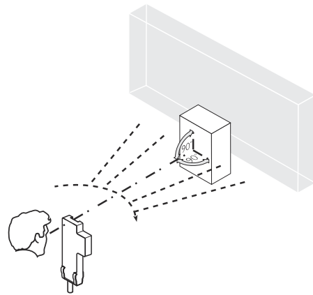
Figure 2: Alignment
