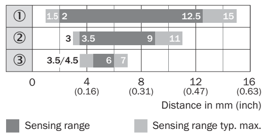
Figure 4: Sensing range 15 mm
