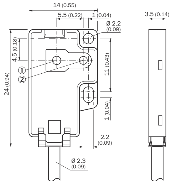
Figure 6: Dimensional drawing GTE2F
