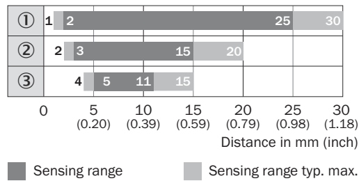
Figure 5: Sensing range 30 mm
