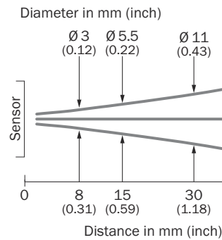
Figure 8: GTE2F, 30 mm version
