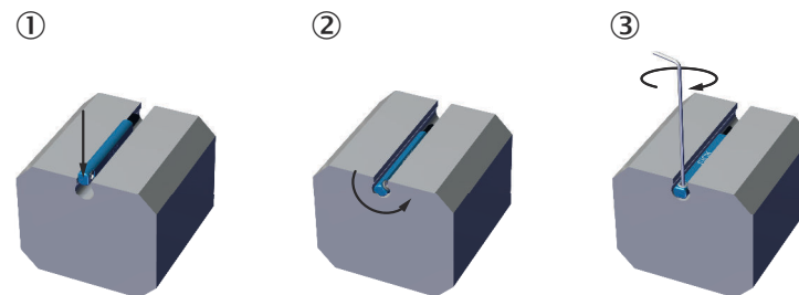
Figure 14: Installation steps
