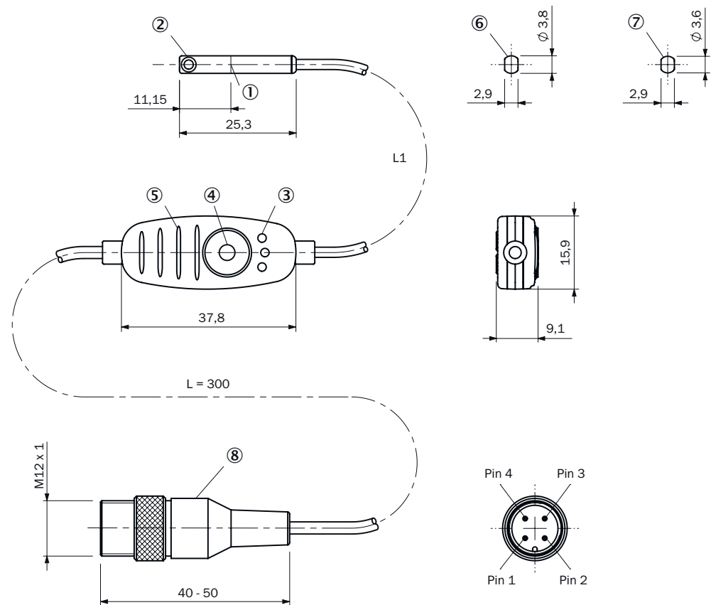
Figure 23: Dimensional drawing with male connector, M12 knurled
