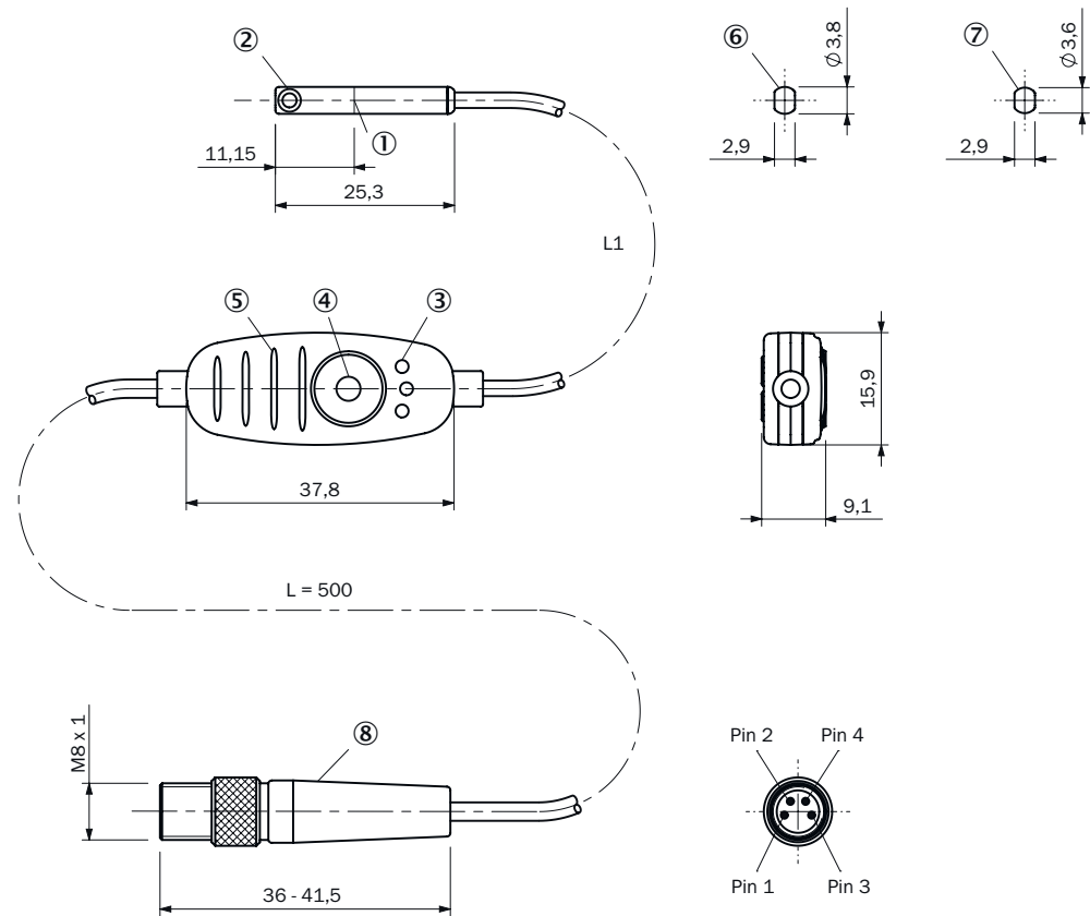
Figure 22: Dimensional drawing with male connector, M8 knurled
