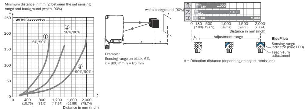
Figure 18: Characteristic line 3, WTB26 I-xxxx1 xx, infra-red light
