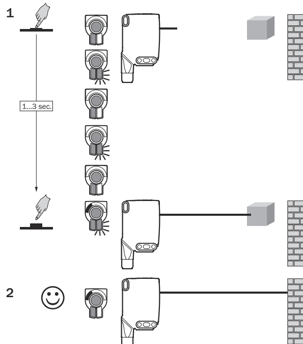
Figure 22: WTB26x-xxxxxx3xAxx, adjusting the sensing range with teach-in button
