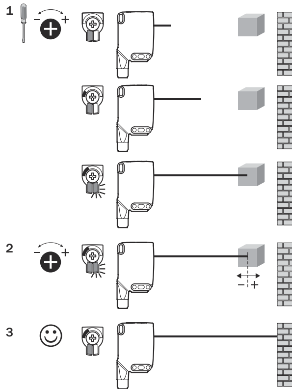
Figure 21: WTB26x-xxxxxx1xAxx, adjusting the sensing range with potentiometer
