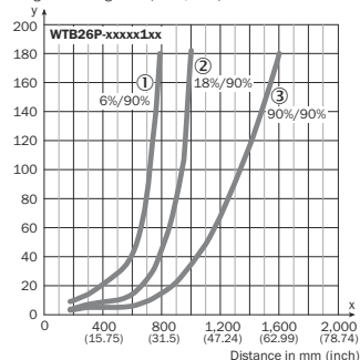
Figure 16: Characteristic line 1, WTB26P-xxxx1xx, red light
