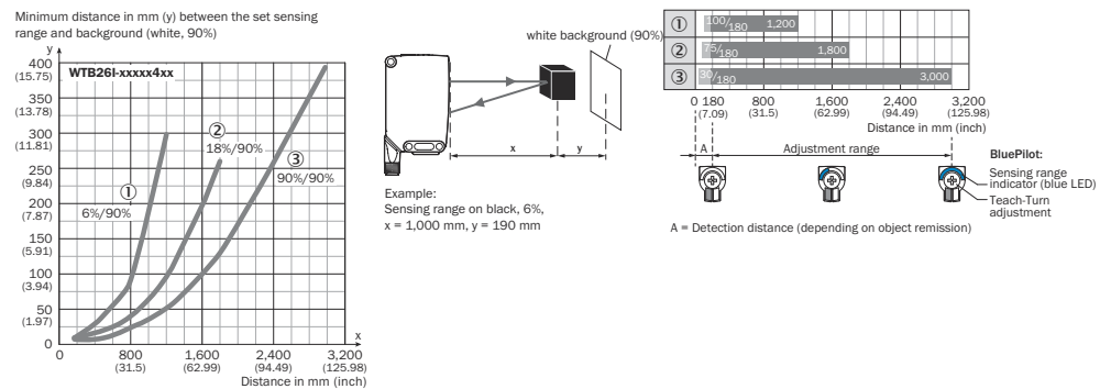
Figure 19: Characteristic line 4, WTB26 I-xxxx4 xx, infra-red light
