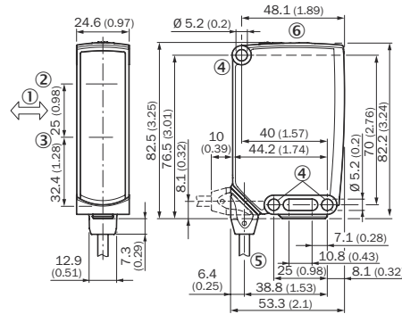
Figure 23: Dimensional drawing 1, cable
