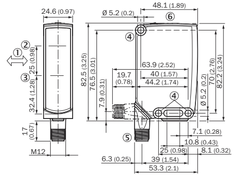
Figure 24: Dimensional drawing 2, male connector
