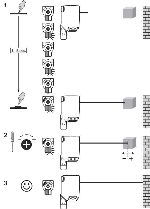
Figure 20: WTB26x-xxxxxx2xAxx, adjusting the sensing range with Teach-Turn adjustment
