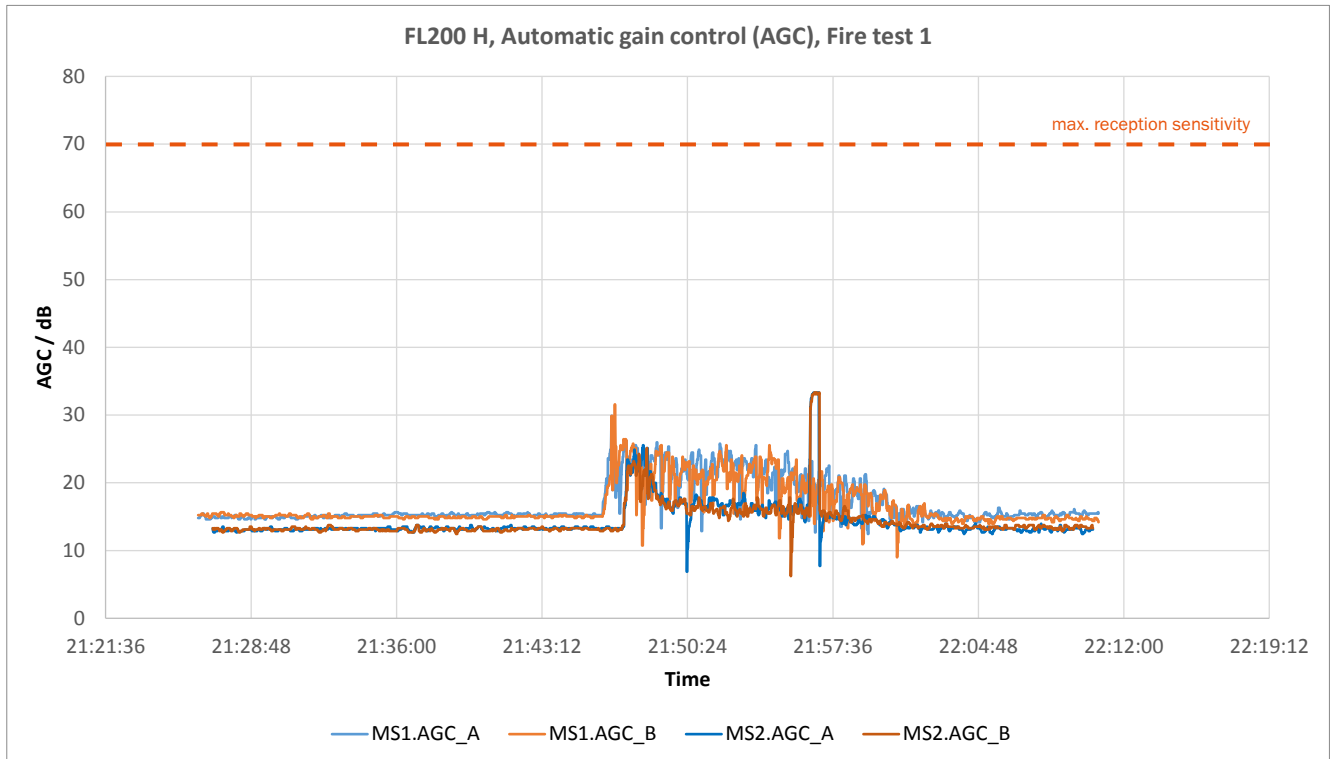
Diagram 7: FL200 H, automatic gain control (AGC), fire test 1, “one-way traffic” operating mode MS1 approx. 25 m downstream behind the fire location MS2 approx. 110 m downstream behind the fire location
