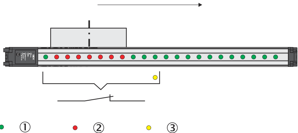
Figure 107: Classification of the object position – object center is smaller than or equal to n beam
