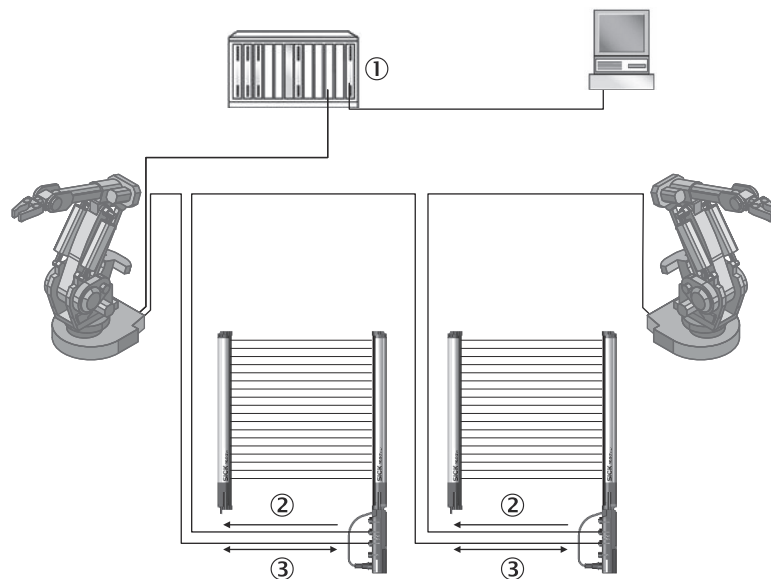
Figure 48: Example of PROFIBUS network in a bus structure (line)
