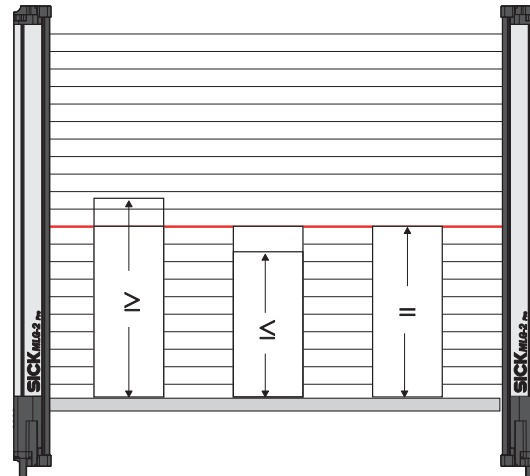
Figure 91: Settings for height classification
