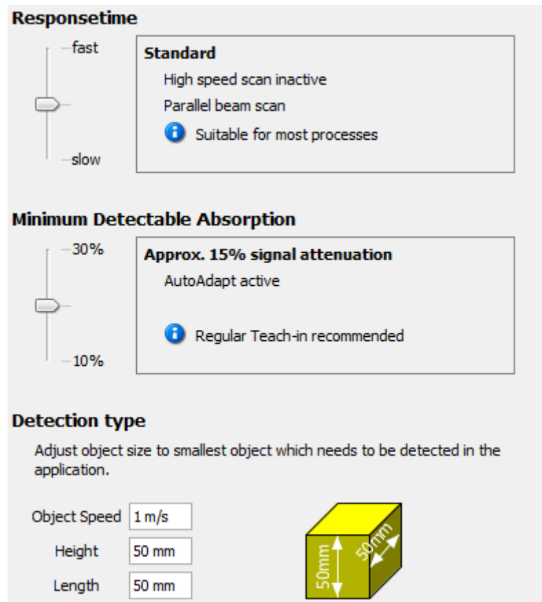
Figure 124: Performance options for Transparent operating mode
