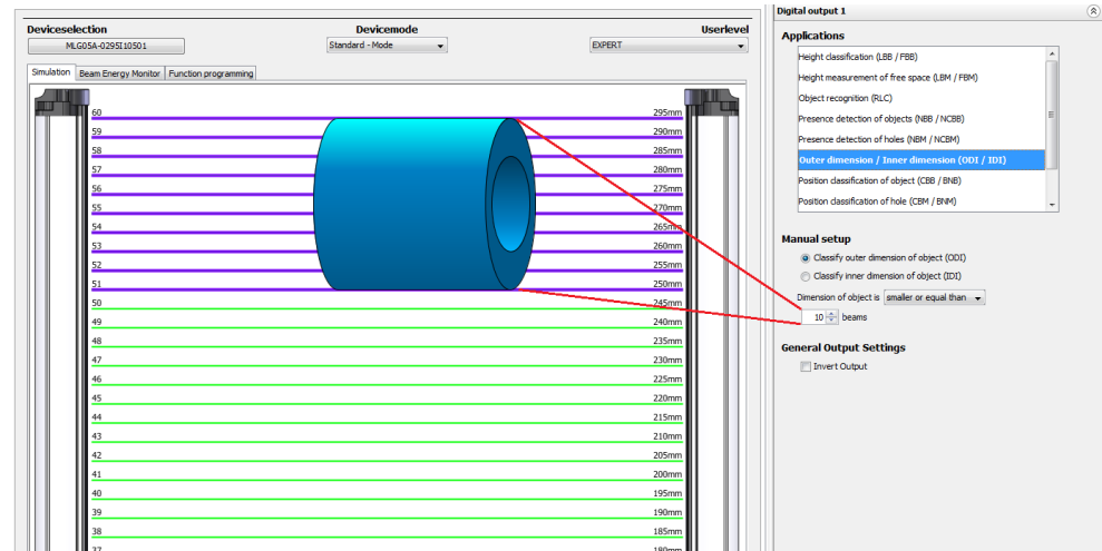
Figure 90: Example representation of the outer dimension
