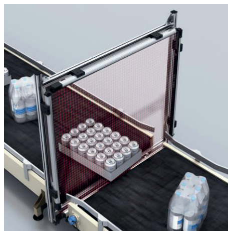
Figure 29: Placement of two light grids at right angles
