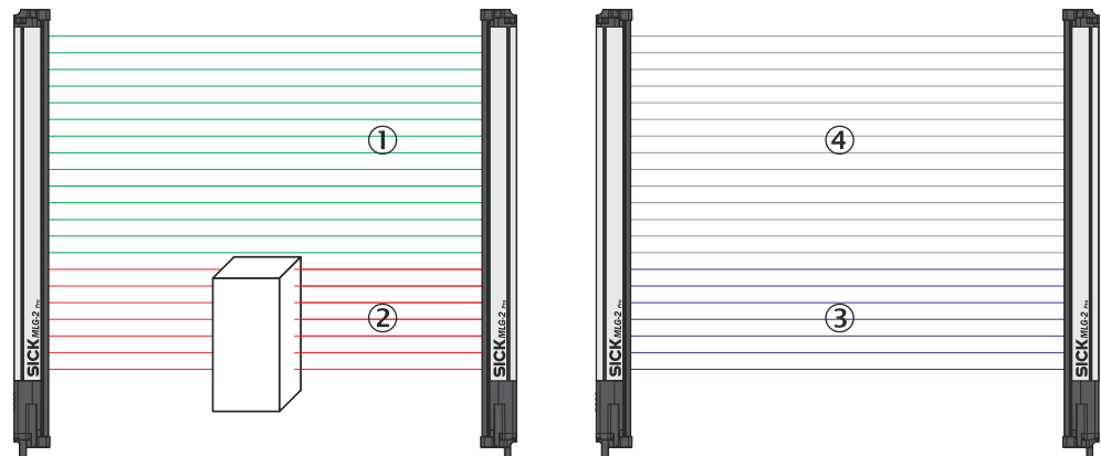
Figure 122: Example of blanking made beams
