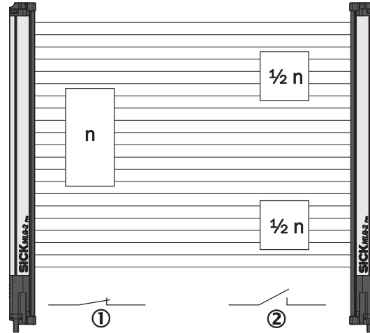
Figure 99: Object detection of consecutive objects
