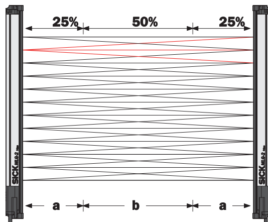
Figure 12: Cross-beam function
