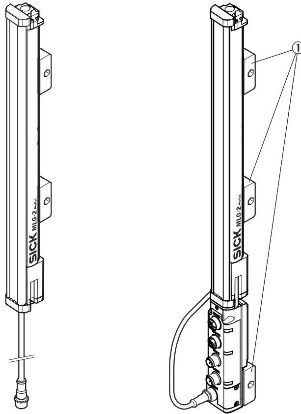
Figure 33: QuickFix bracket for the fieldbus module
