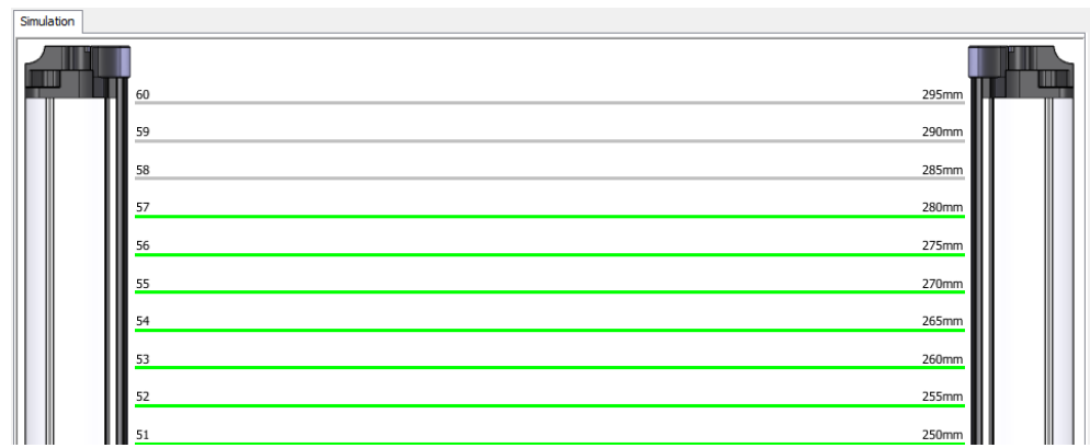
Figure 81: Blanked beams
