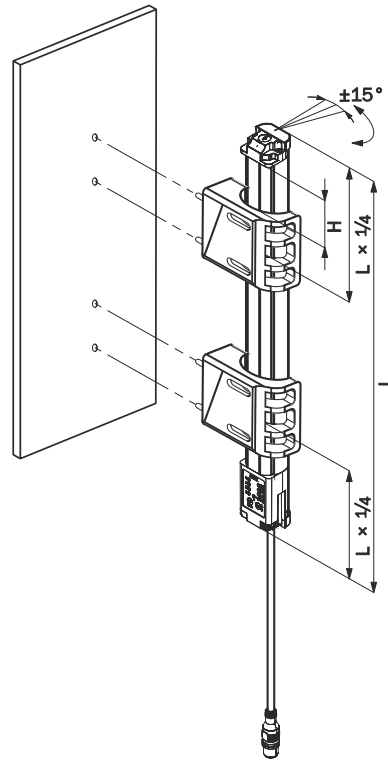
Figure 45: Alignment with the FlexFix bracket
