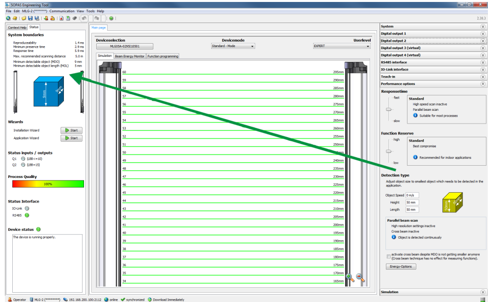
Figure 86: Effects of the performance options on the system boundaries
