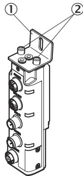
Figure 40: Mount the fieldbus module offset using the mounting bracket
