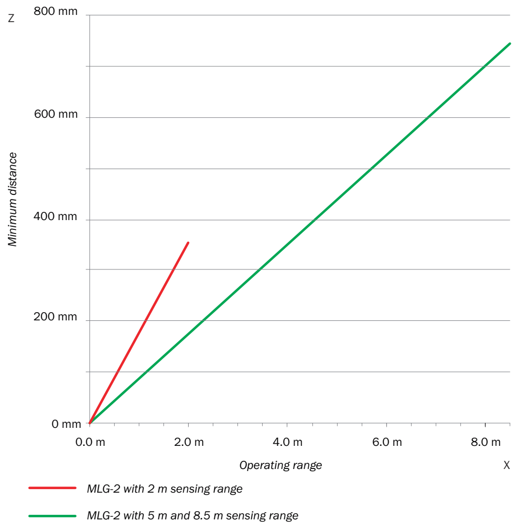
Figure 28: Graph, distances when light is in the same direction (XZ)
