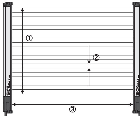
Figure 2: Detection area of the MLG-2
