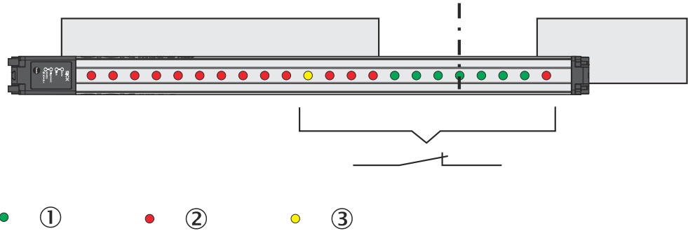
Figure 110: Classification of the hole position – larger than or equal to hole center
