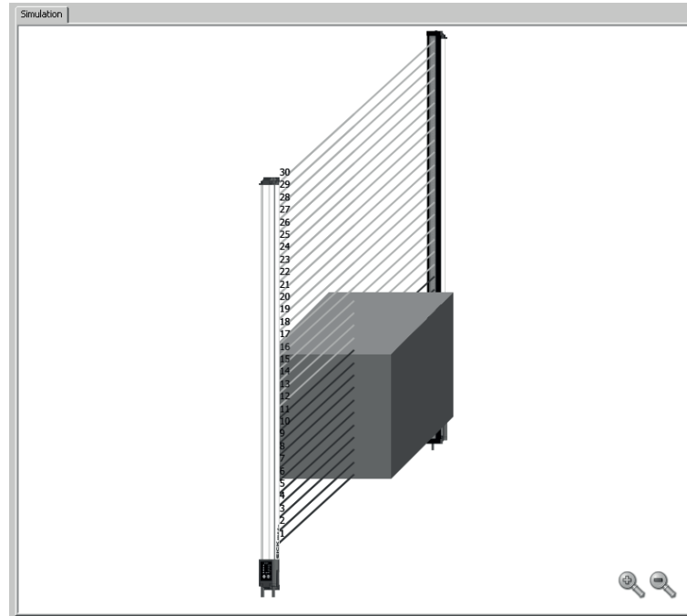
Figure 136: Simulation object in Simulation area
