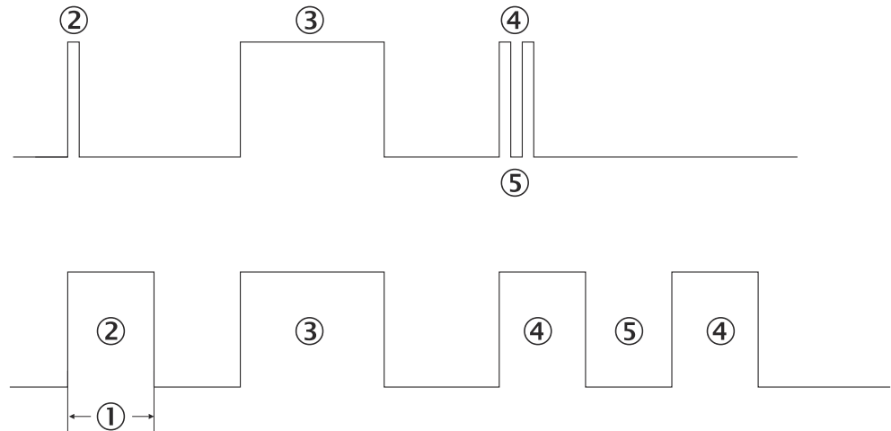
Figure 114: Examples of the effect of a configured minimum pulse width
