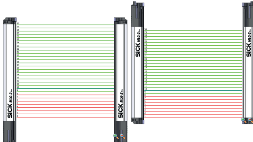
Figure 68: Beam numbering
