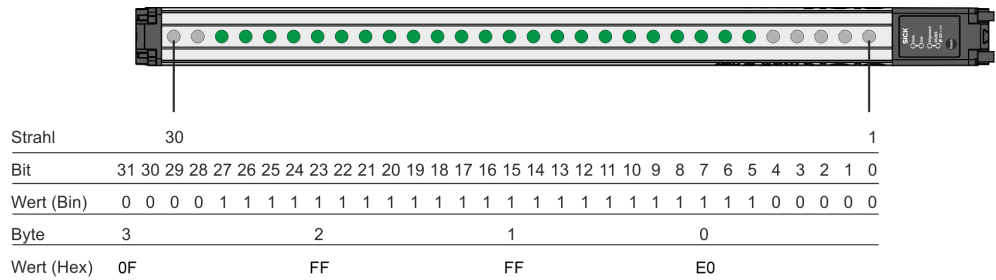
Figure 67: Bit-coded beam mask for an MLG-2, with 30 beams
