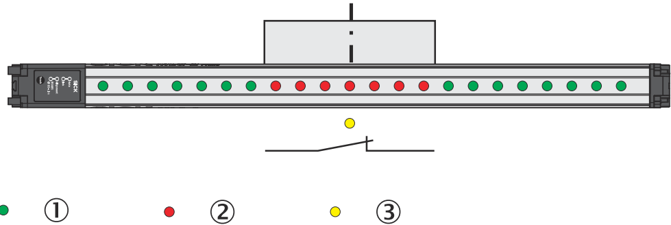
Figure 108: Classification of the object position – object center is equal to n beam
