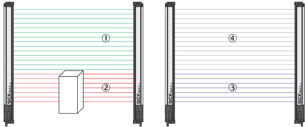
Figure 66: Example of blanking made beams
