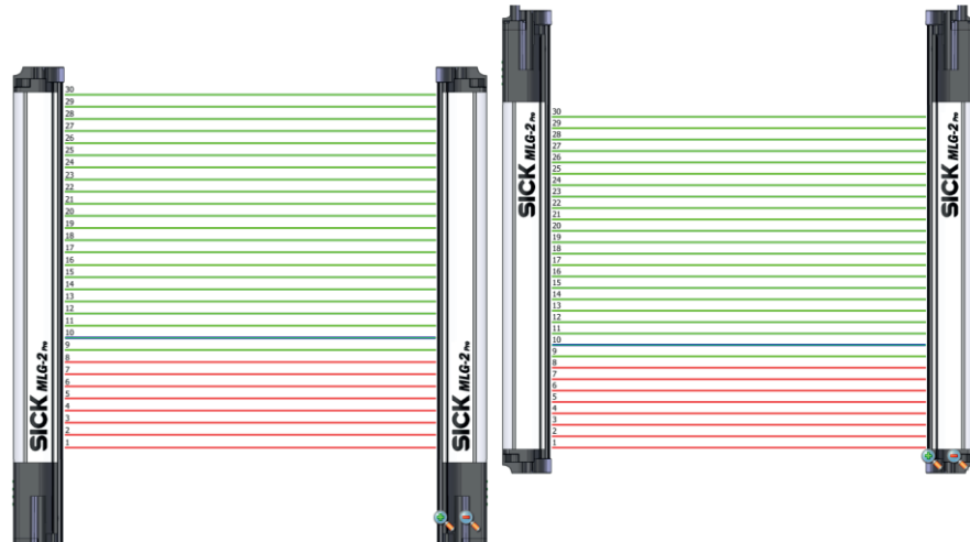
Figure 88: Beam numbering
