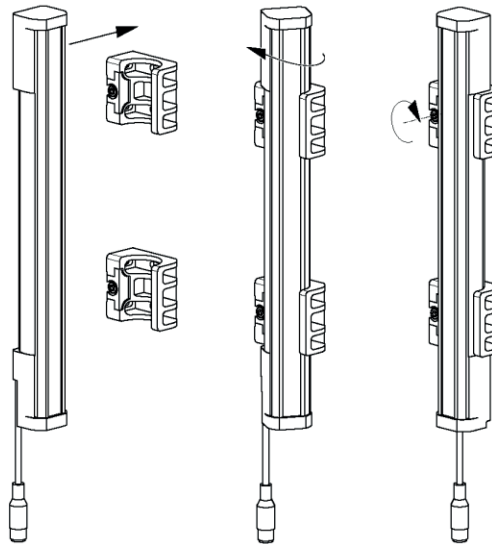
Figure 35: Inserting the MLG-2 in the FlexFix brackets
