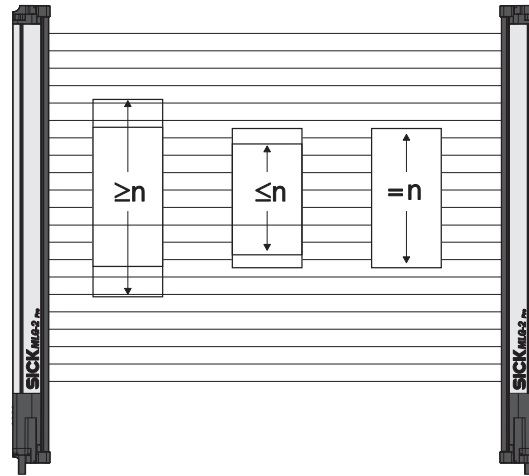
Figure 97: Object detection/object width
