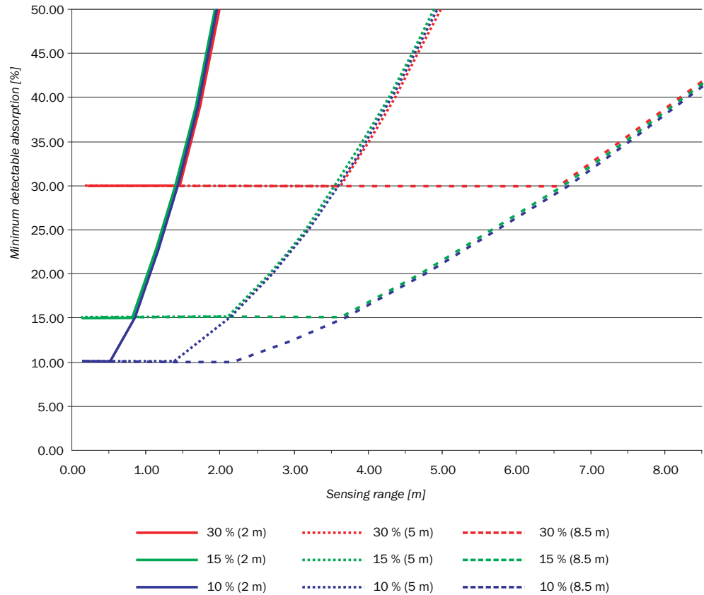
Figure 144: Minimum detectable absorption required for devices with 2 m, 5 m and 8.5 m sensing range
