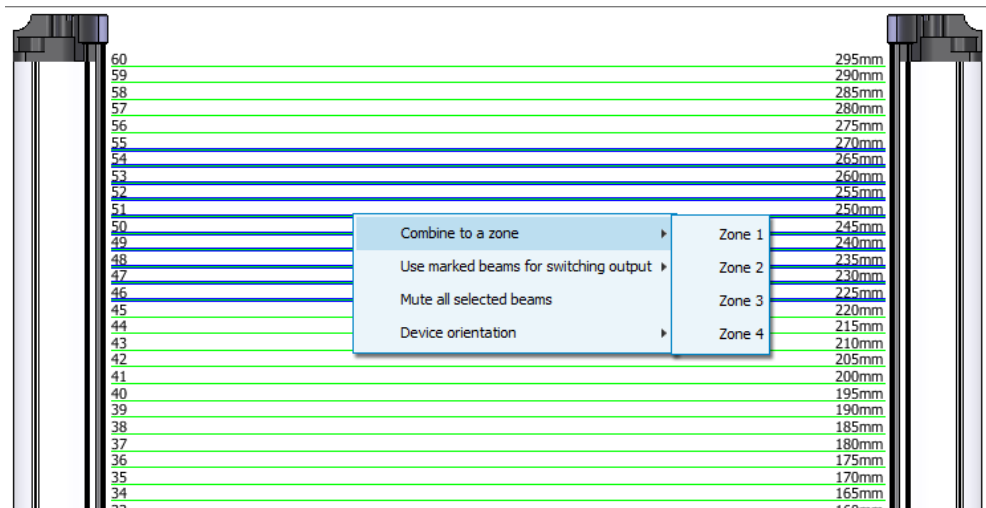
Figure 76: Combining beams into zones
