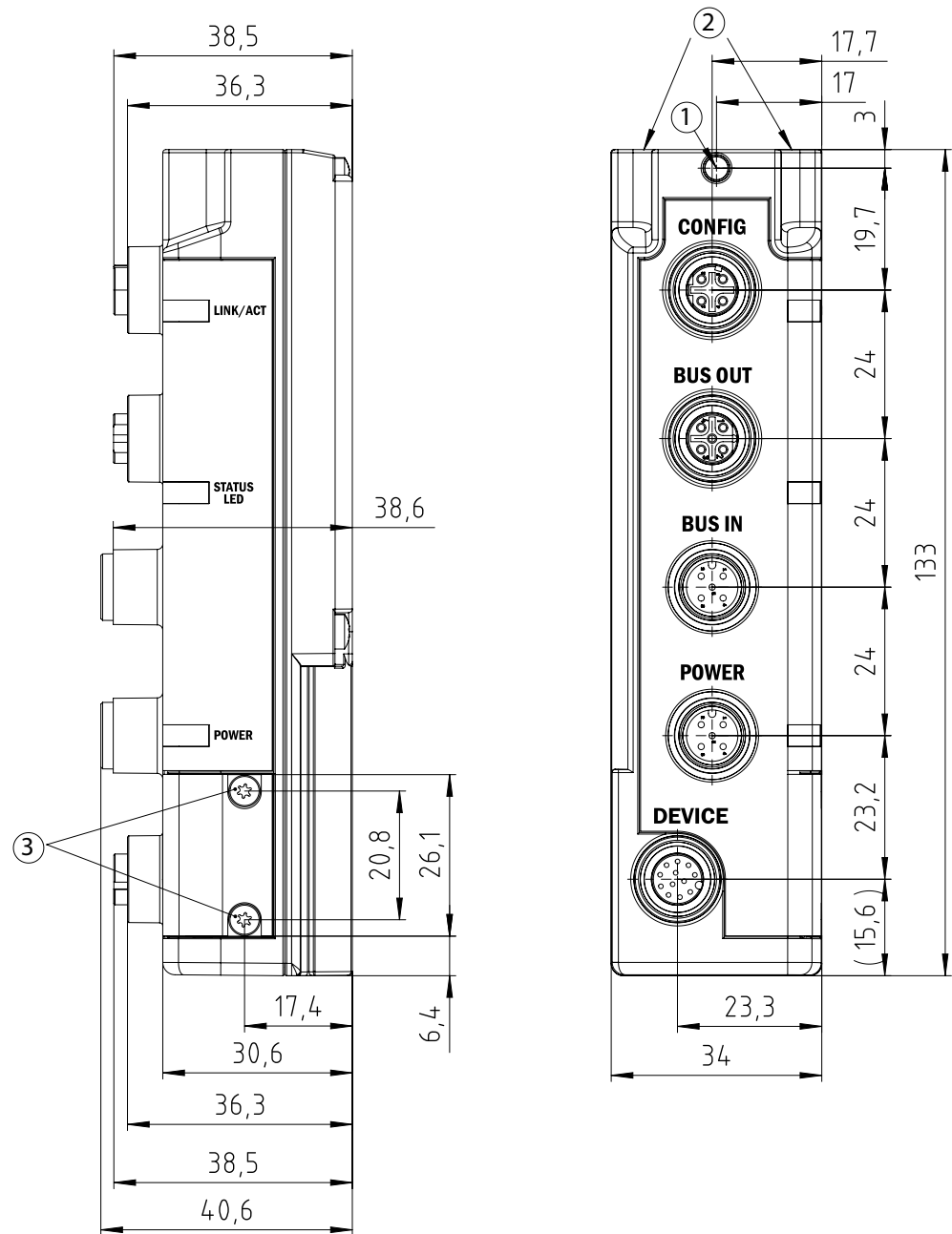
Figure 147: Dimensional drawing 2 MLG-2 fieldbus module
