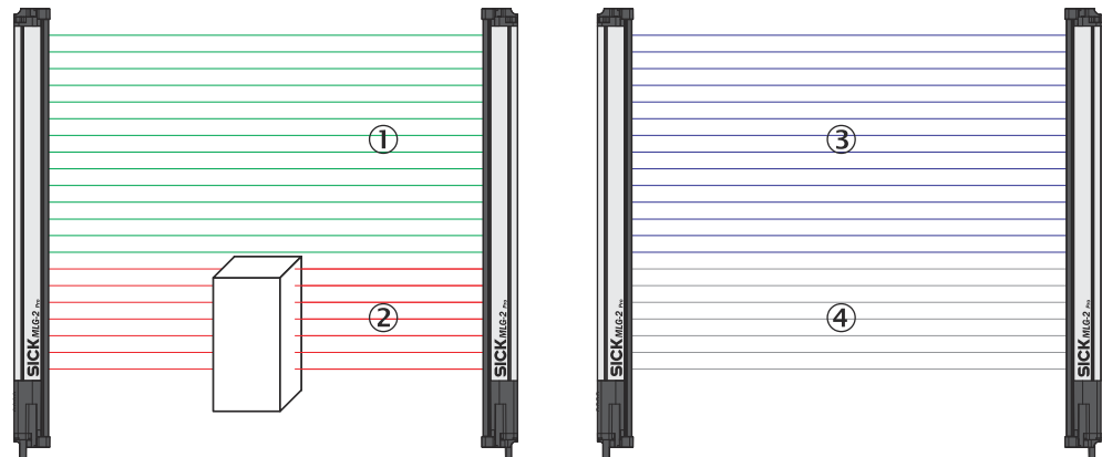
Figure 65: Example of the blanking of blocked beams
