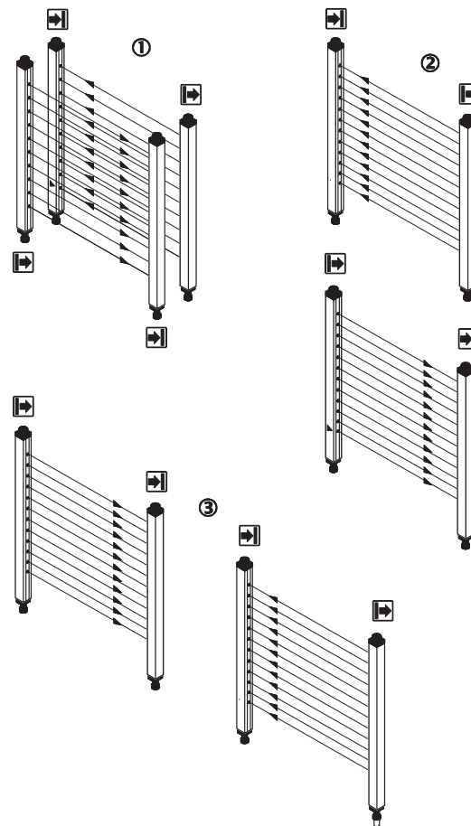
Figure 25: Placement with light in opposite directions
