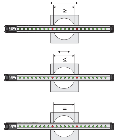
Figure 104: Measurement of the inside dimension
