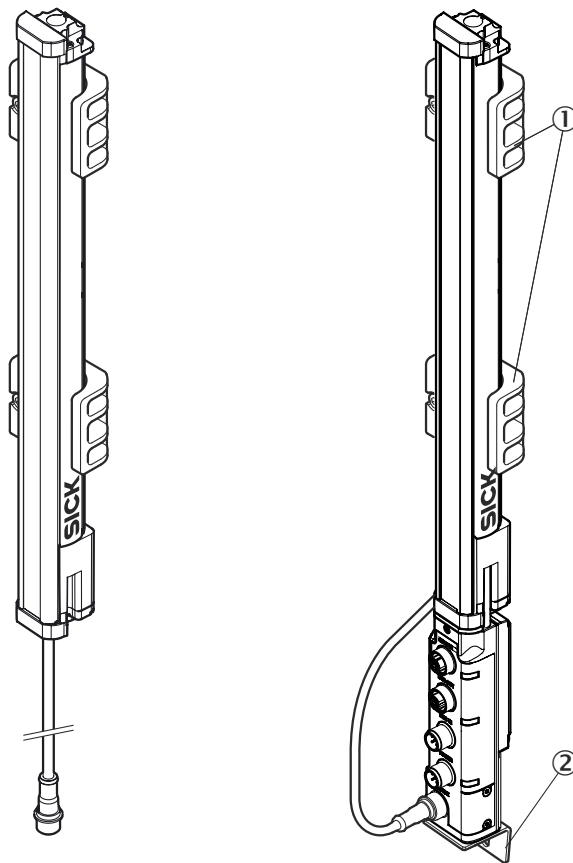
Figure 36: Mounting bracket for the fieldbus module
