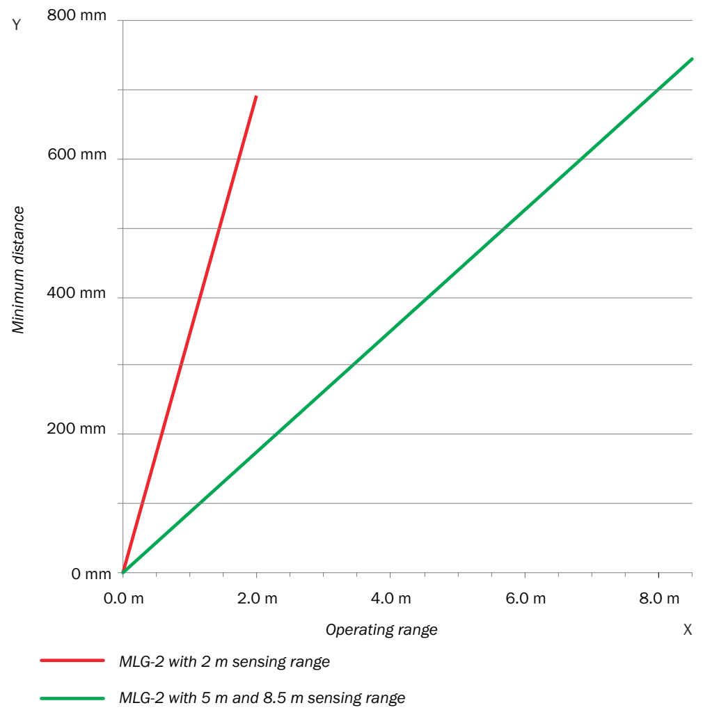
Figure 27: Graph, distances when light is in the same direction
