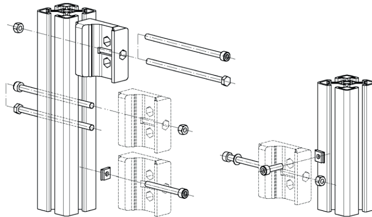
Figure 32: Mount QuickFix bracket to a profile frame
