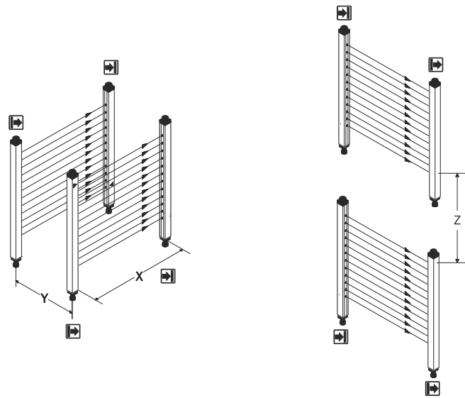
Figure 26: Distances when light is in the same direction
