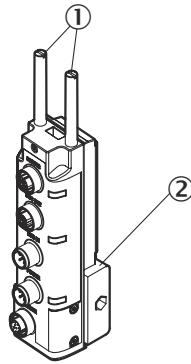
Figure 39: Mount the fieldbus module offset using the QuickFix bracket
