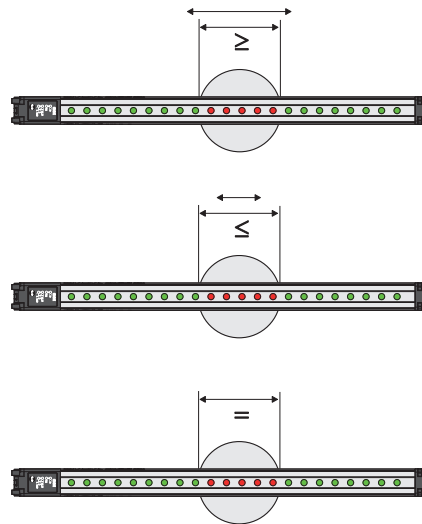
Figure 103: Measurement of the outside dimension
