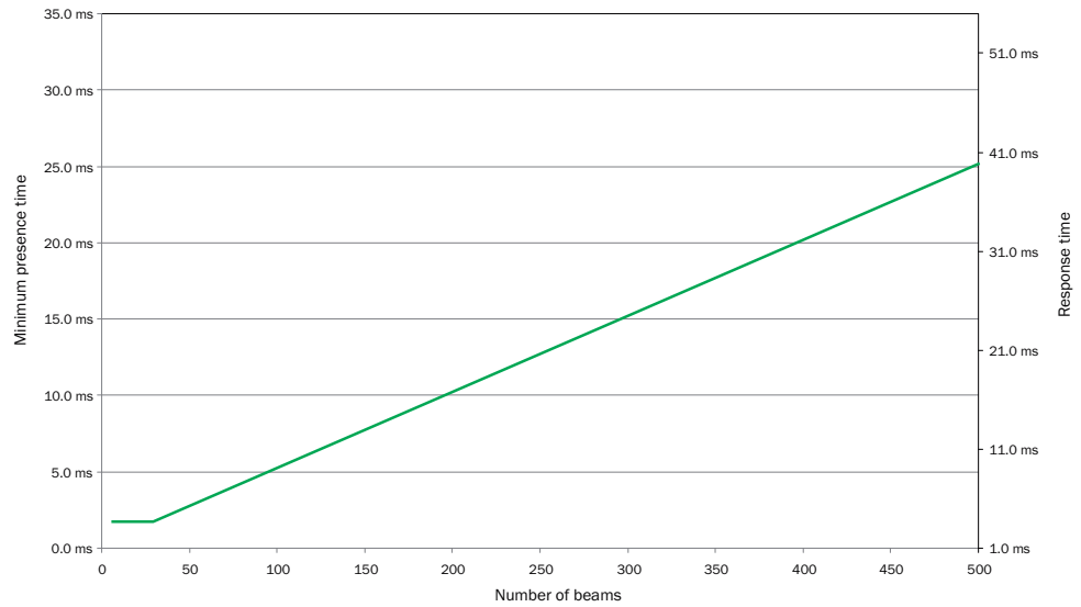
Figure 140: Graph, MLG-2 Pro response time and minimum presence time
