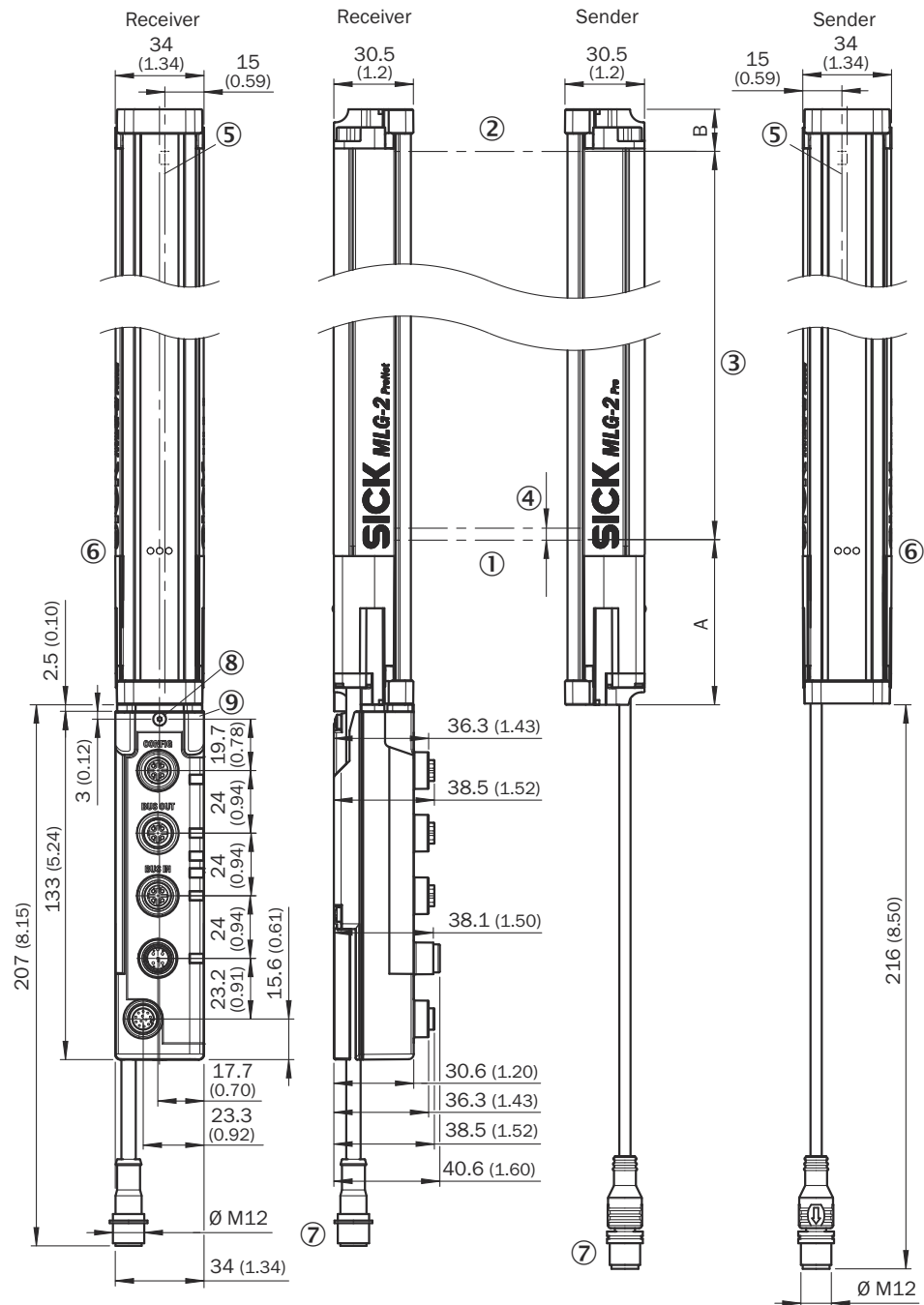
Figure 145: Dimensional drawing MLG-2 ProNet (mm)
