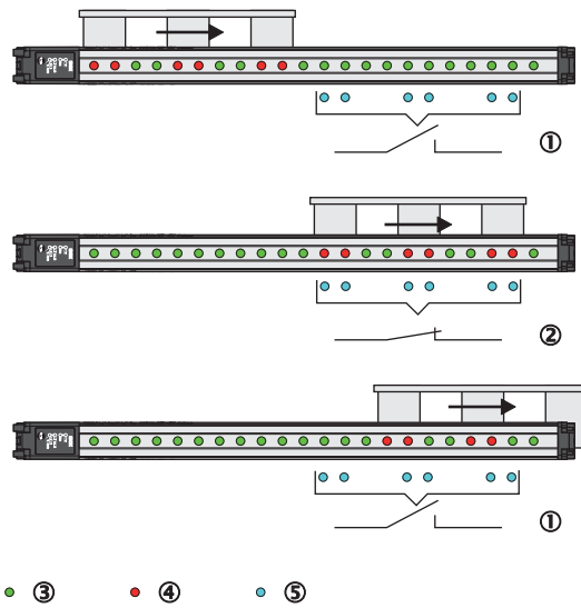
Figure 94: Object recognition, static
