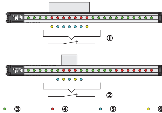
Figure 96: Object recognition with tolerance
