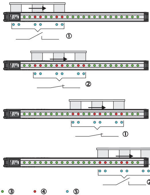
Figure 95: Object recognition, dynamic
