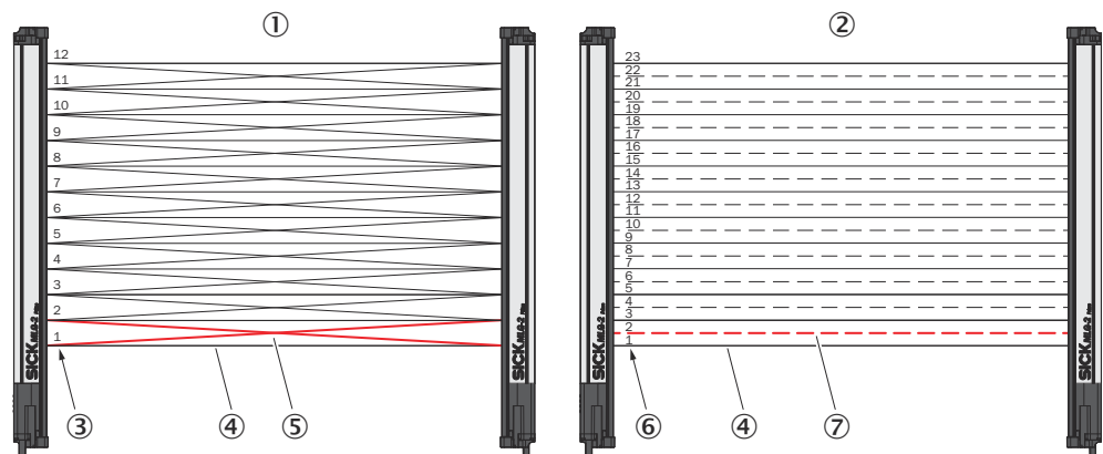
Figure 126: Left: “Cross beam switching”, right: “Cross beam measuring”
