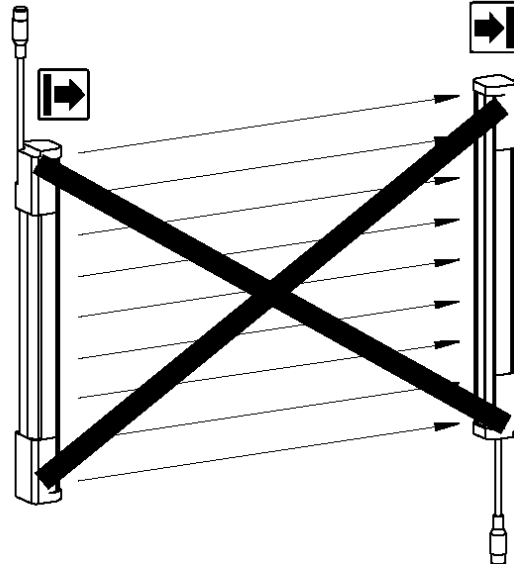
Figure 31: The sender and receiver are aligned incorrectly
