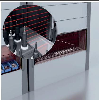
Figure 21: Detection of small objects
