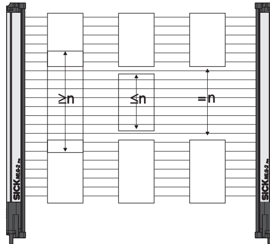
Figure 100: Hole detection/hole size
