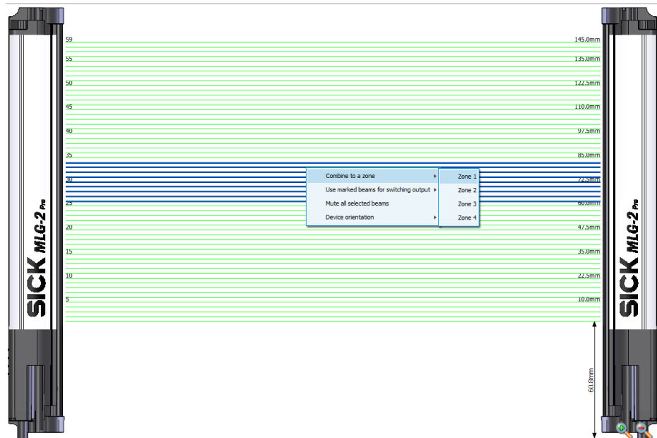
Figure 116: SOPAS ET beam window – Combining beams into zones
