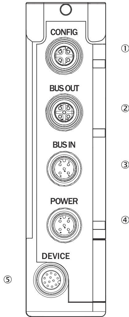
Figure 41: Fieldbus module connections
