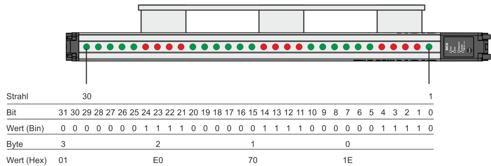
Figure 64: Beam status – Example 2
