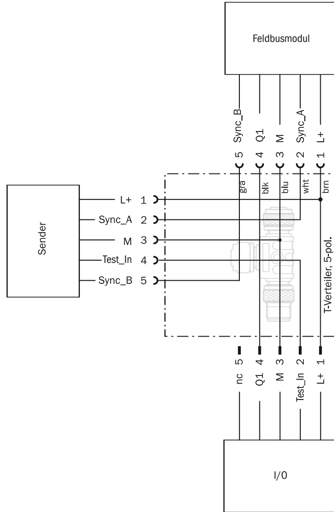
Figure 43: T-connector for sender and fieldbus module
