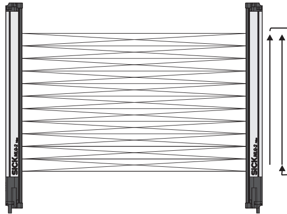
Figure 7: Cross-beam function
