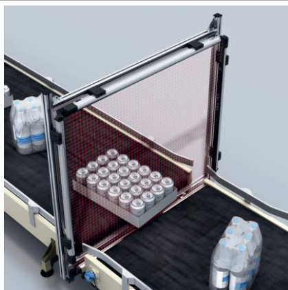
Figure 23: Volume measurement
