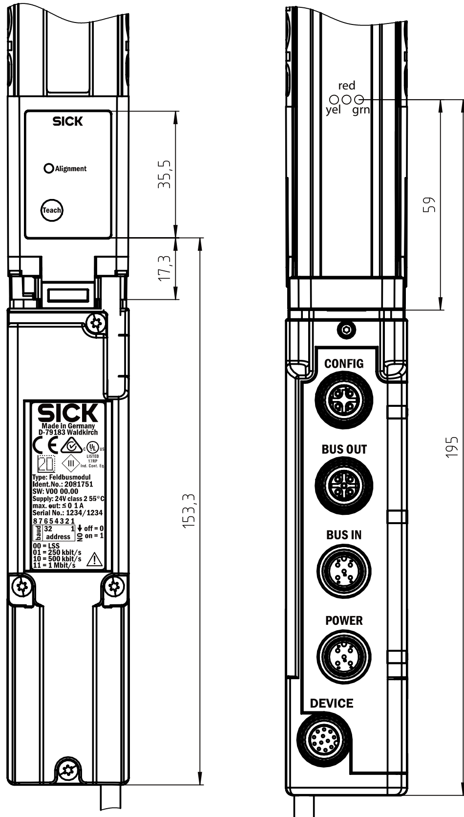
Figure 146: Dimensional drawing 1 MLG-2 fieldbus module
