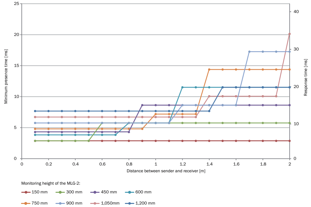
Figure 141: Response time and minimum presence time up to 2 m sensing range
