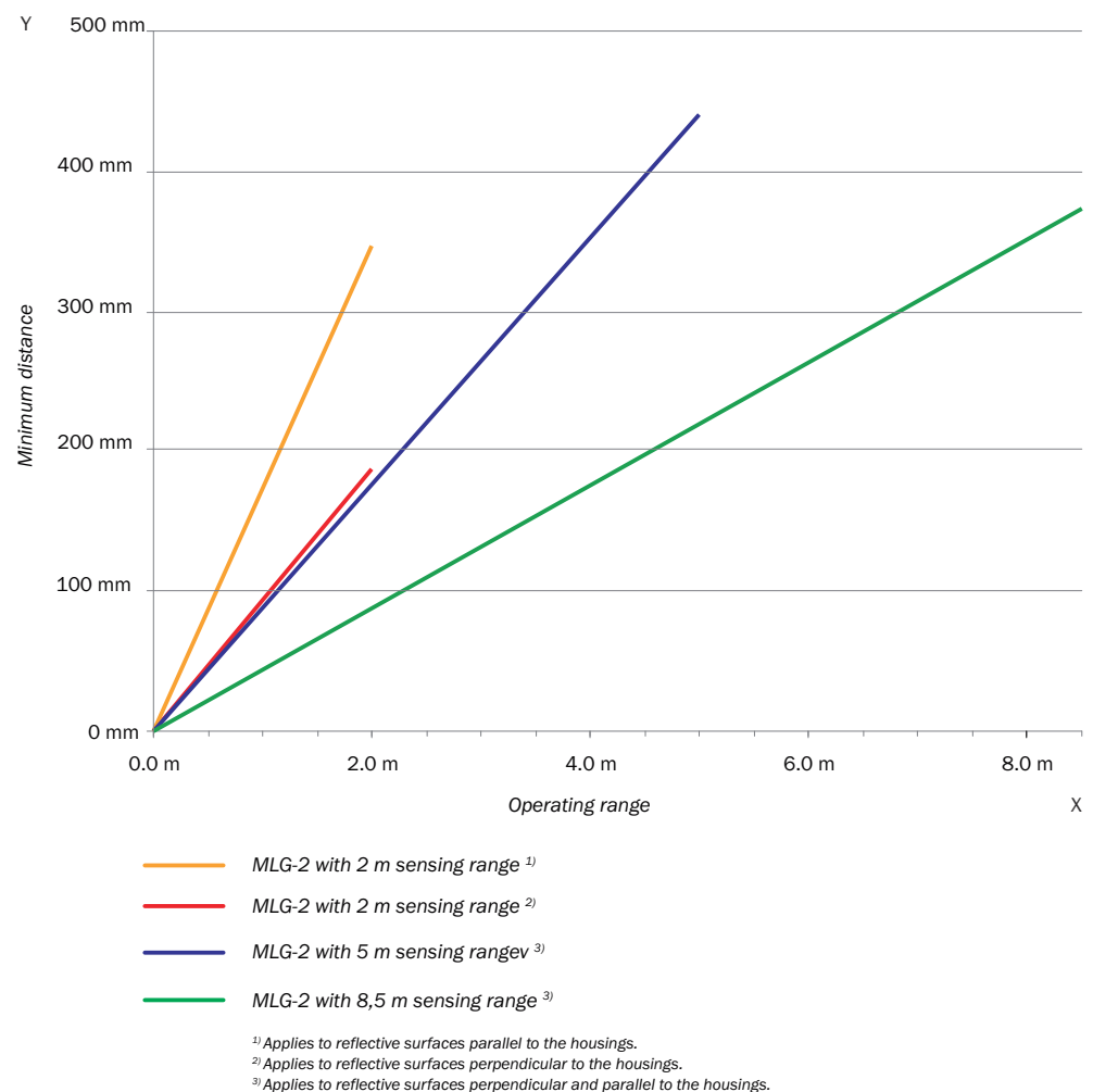
Figure 30: Graph, minimum distance from reflective surfaces
