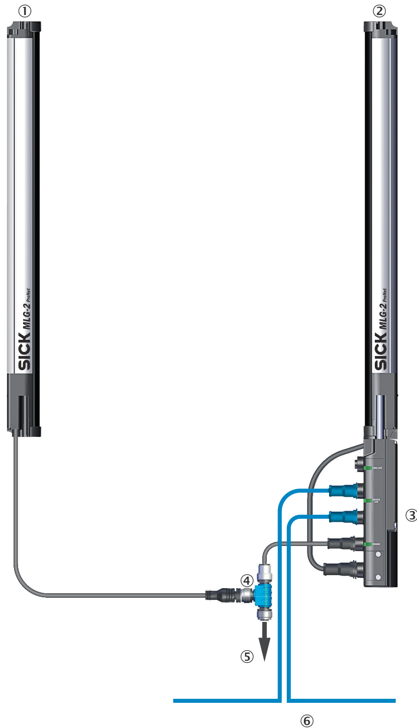
Figure 42: Connection to the PROFIBUS fieldbus
