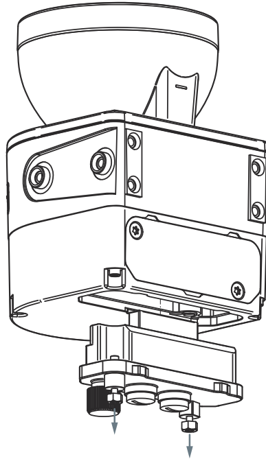
Figure 83: Replacing the system plug
