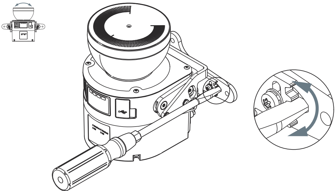
Figure 77: Alignment about the depth axis
