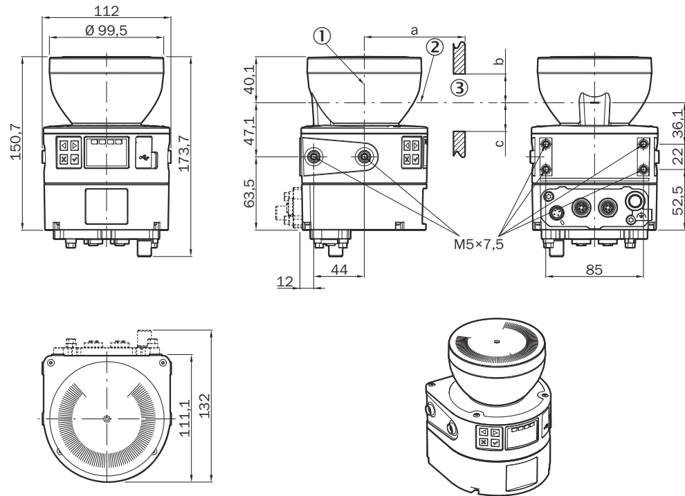
Figure 93: Dimensional drawing
