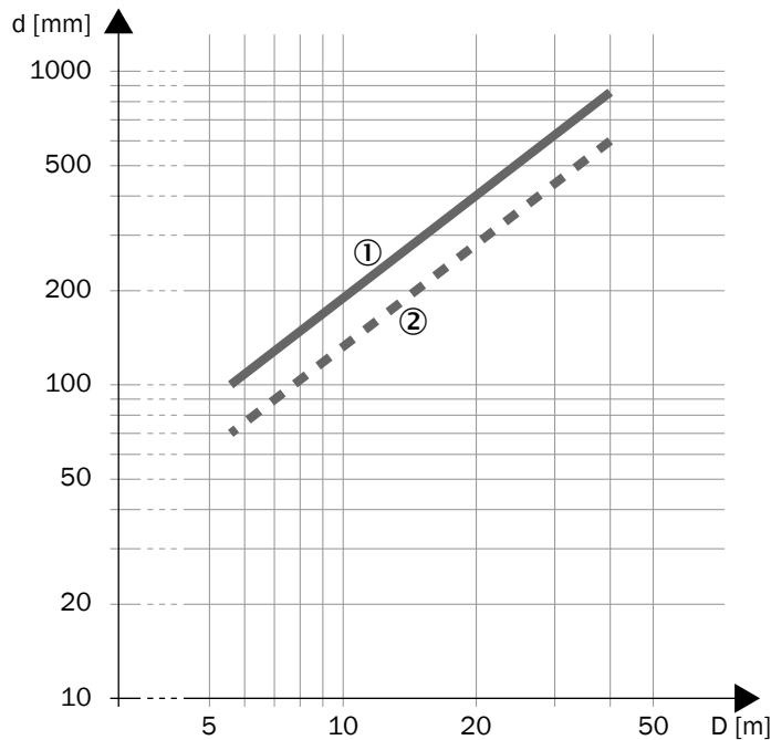
Figure 89: Scanning range and object size for warning fields (devices with a max. protective field range of 4.0 m and devices with max. protective field range of 5.5 m)
