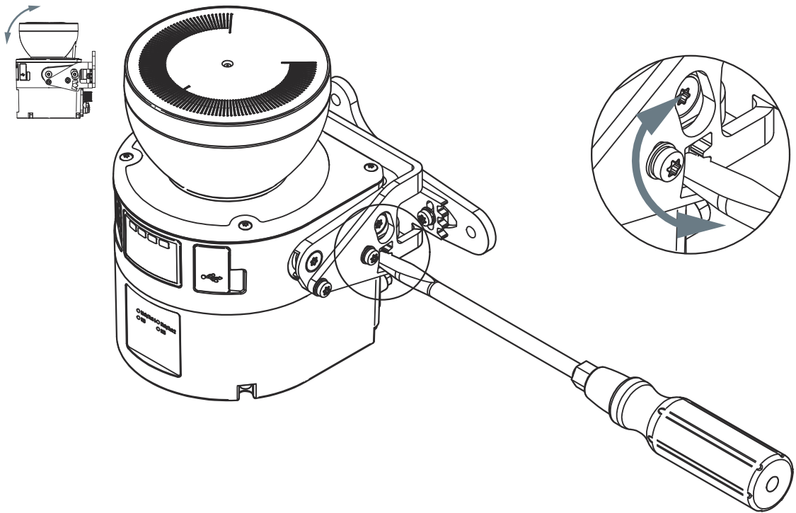
Figure 76: Alignment about the transverse axis
