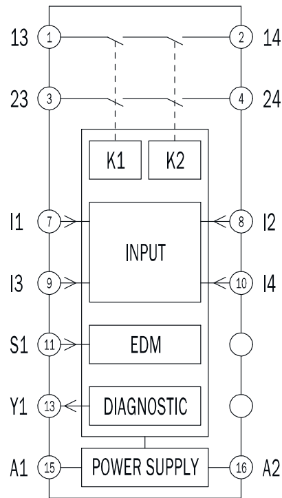
Figure 14: Internal circuitry
