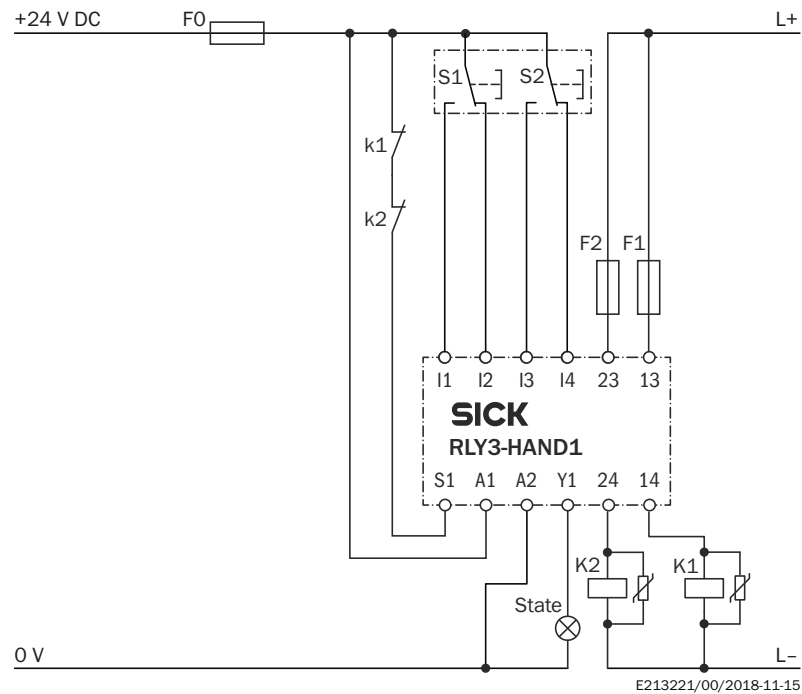
Figure 4: ReLy HAND1 connection diagram
