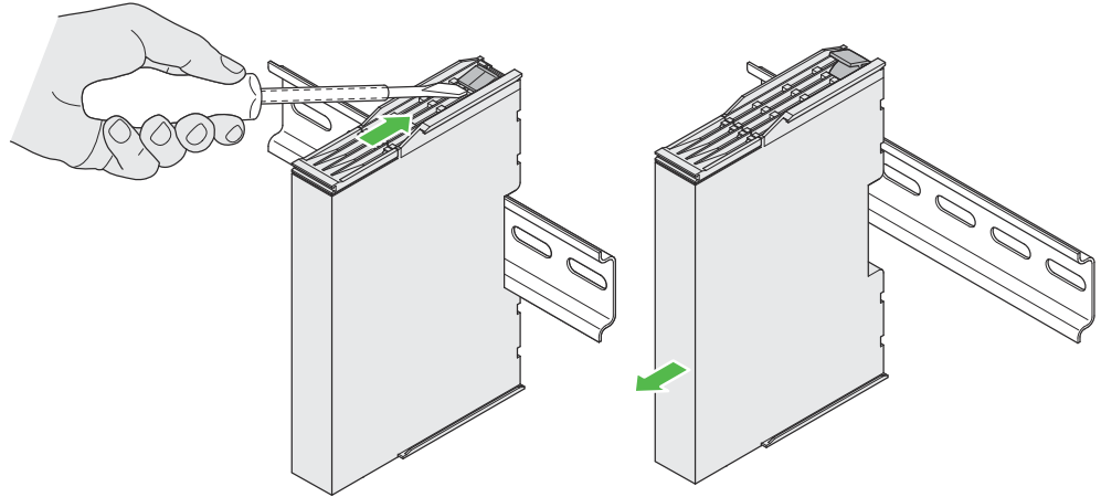
Figure 7: Disassembly
