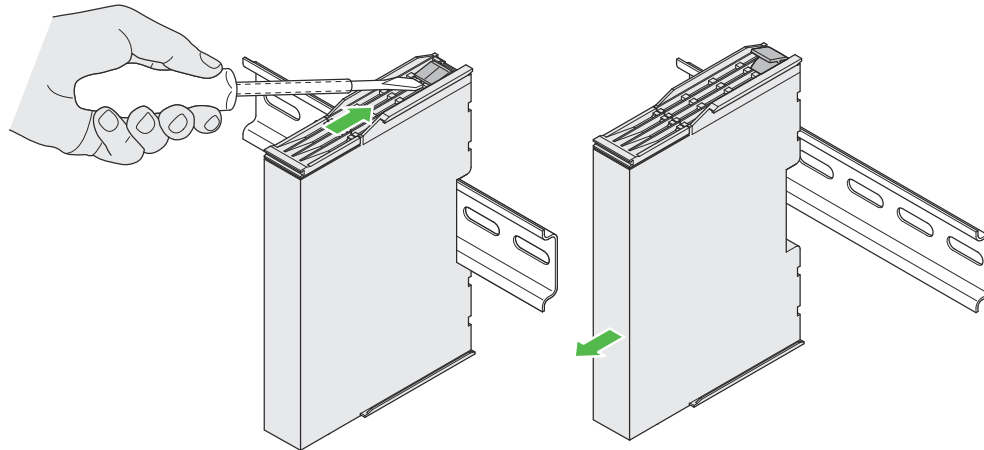
Figure 9: Disassembly
