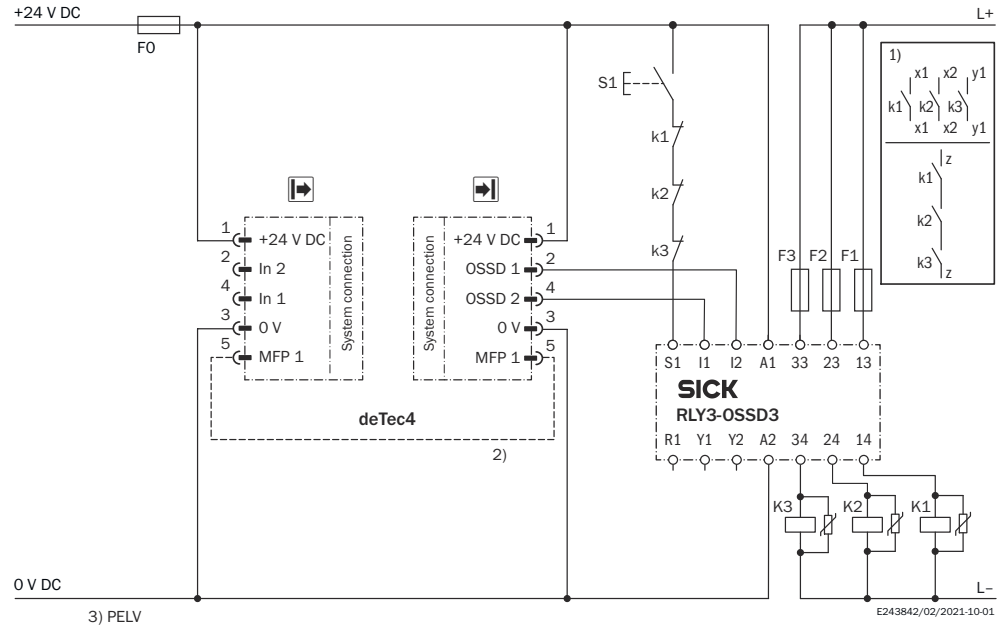
Figure 5: ReLy OSSD3 connection diagram, with restart interlock and external device monitoring (EDM)
