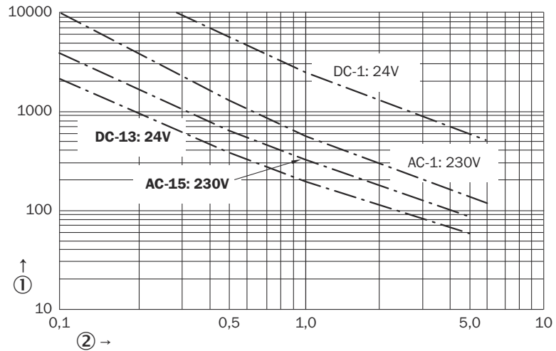
Figure 14: Electrical endurance of contacts 13/14, 23/24 and 33/34
