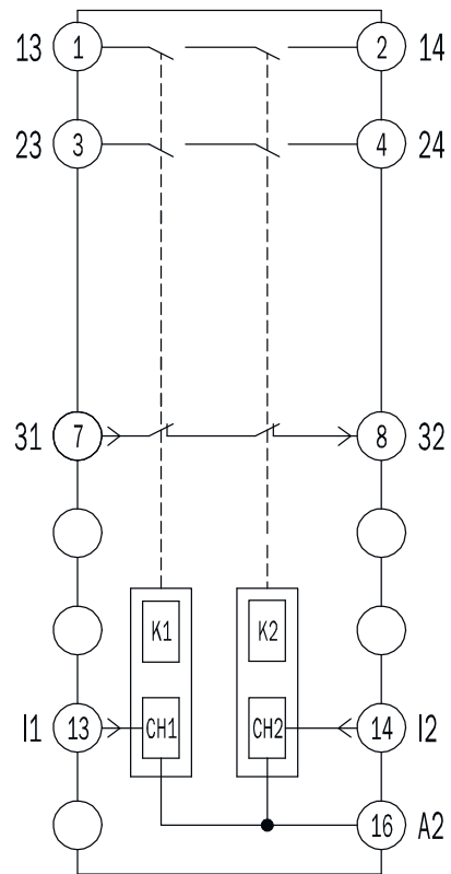
Figure 13: Internal circuitry (hardware version 1.11.0 and above)
