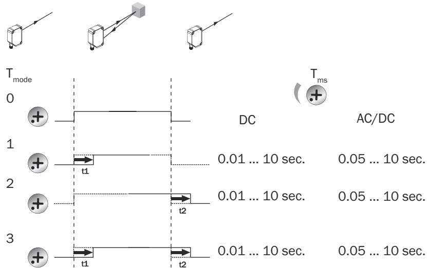
Figure 11: Time functions
