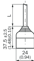
Figura 18: Conector Q7
