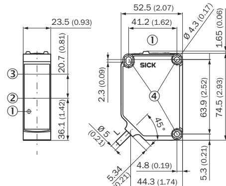
Illustration 14: GTE20, câble
