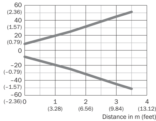
Figure 20: Light spot size, infrared light
