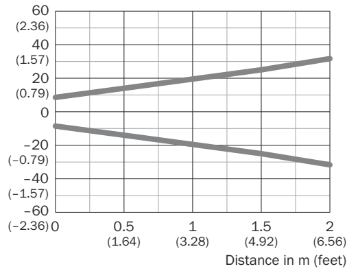
Figure 19: Light spot size, red light
