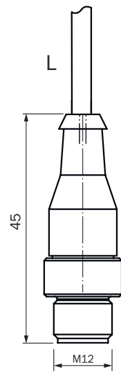
Figure 16: Connector M12
