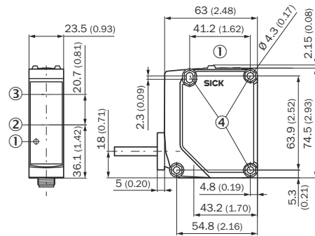
Figure 15: GTE20, Terminal chamber
