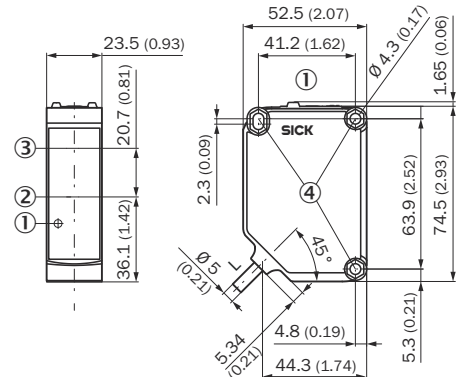
Figure 14: GTE20, Cable
