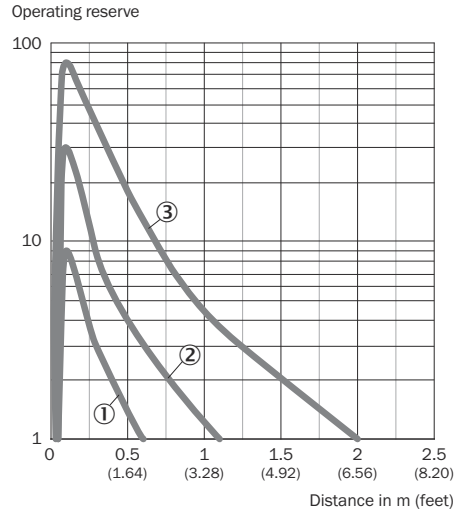
Figure 5: Characteristic curve, GTE20G, red light
