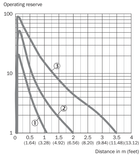
Figure 7: Characteristic curve, GTE20M, infrared light
