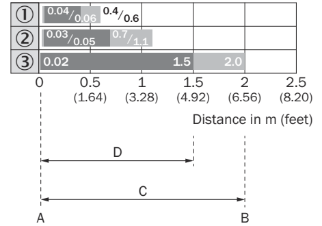
Figure 6: Sensing range diagram, GTE20G, red light
