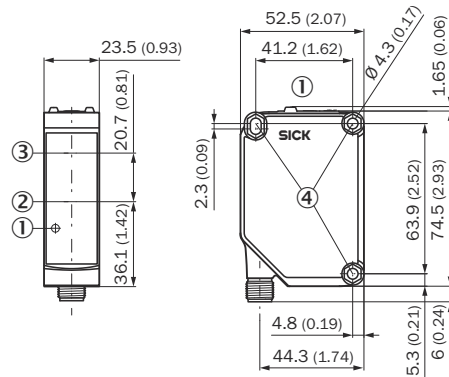
Figure 13: GTE20, M12 connector
