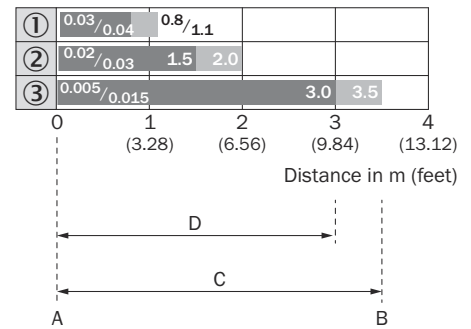
Figure 8: Sensing range diagram, GTE20M, infrared light
