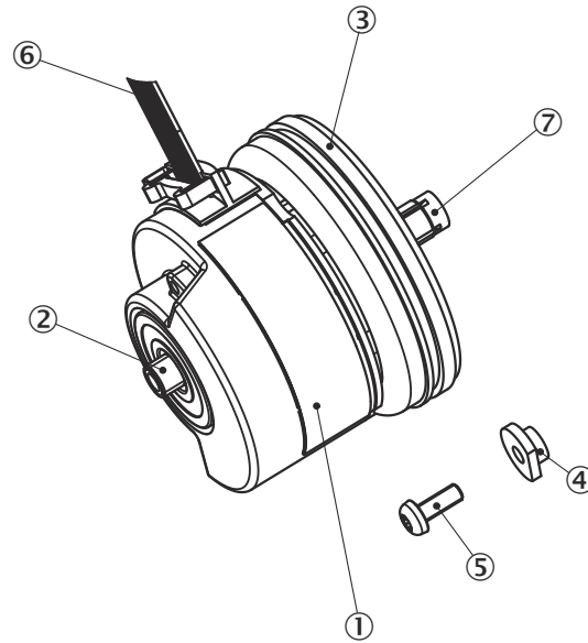
Figure 1: Motor feedback system with plug-in shaft and resolver style support
