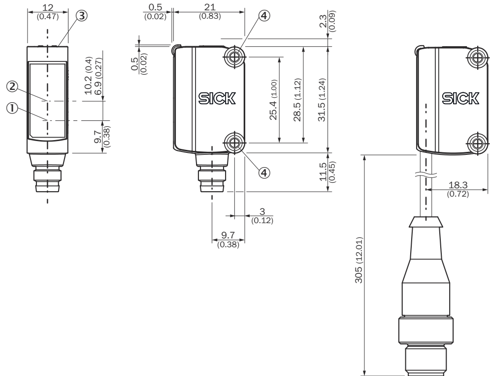
Figure 7: Dimensional drawing
