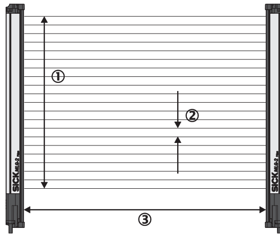
Figure 2: Detection area of the MLG-2
