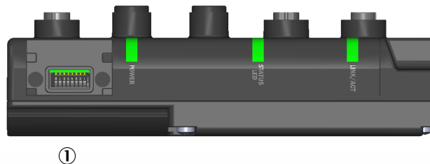
Figure 18: DIP switch on the fieldbus module
