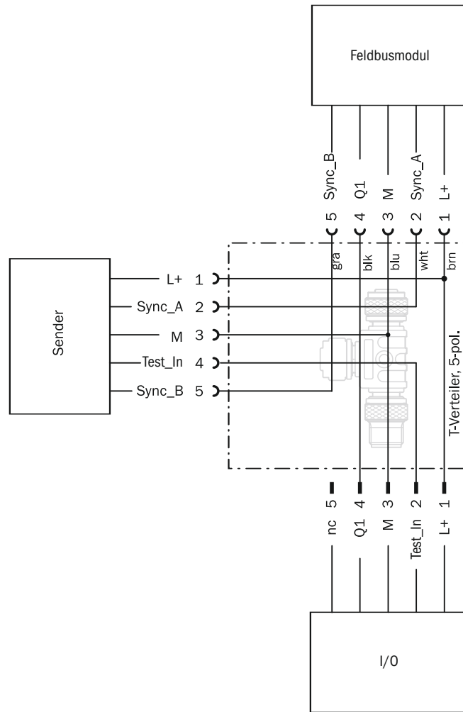
Figure 43: T-distributor of sender and fieldbus module
