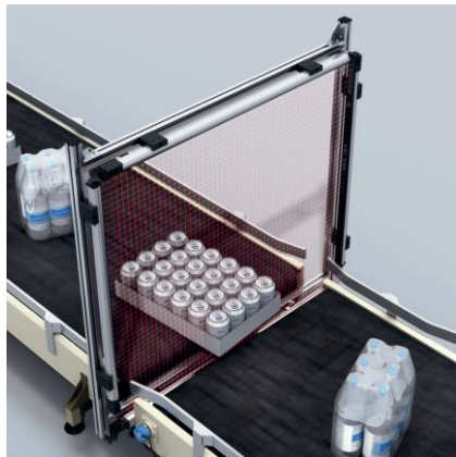
Figure 23: Volume measurement
