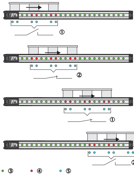
Figure 98: Object recognition, dynamic
