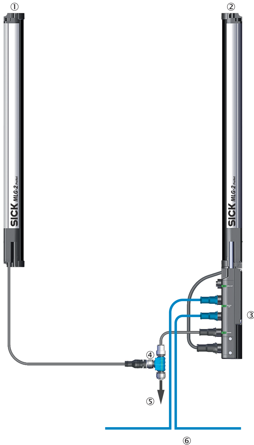
Figure 42: Connection with T-distributor
