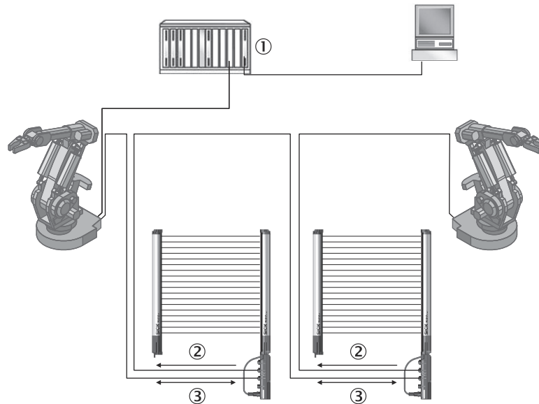
Figure 49: Example of a CANopen network in a line structure
