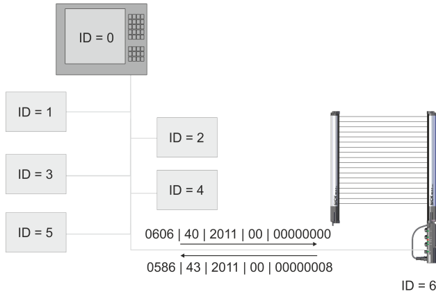
Figure 52: Example of a Receive SDO and a Transmit SDO
