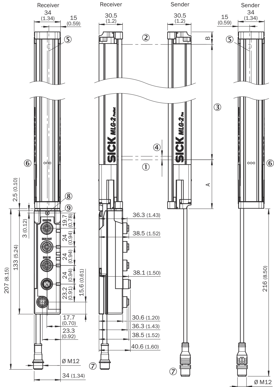
Figure 148: Dimensional drawing MLG-2 ProNet (mm)
