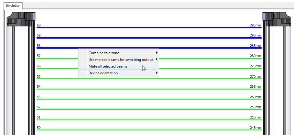
Figure 83: Blanking beams
