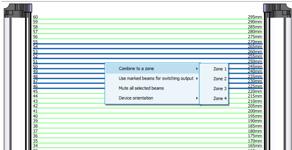
Figure 79: Combining beams into zones
